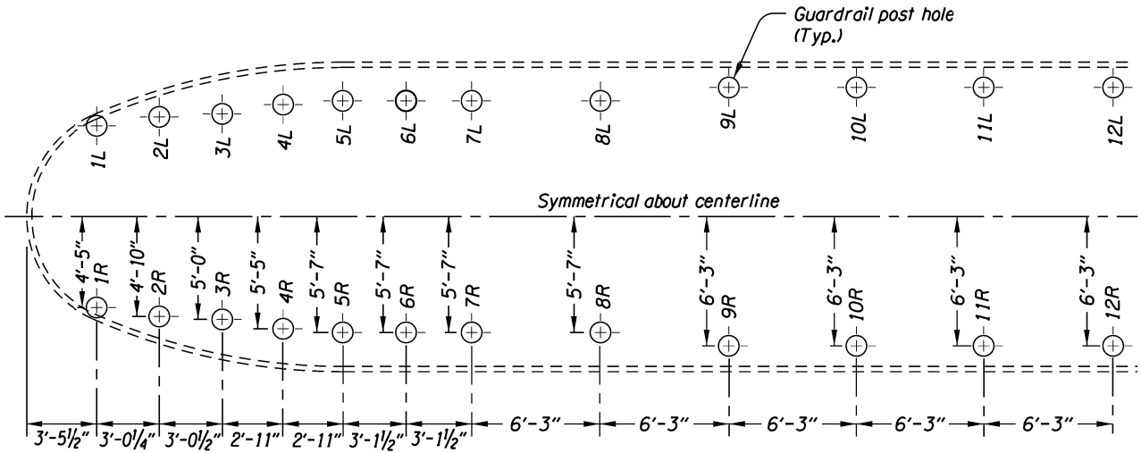
PLAN GUARDRAIL POST LAYOUT - DESIGN 1
