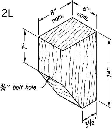
TAPERED BLOCK
