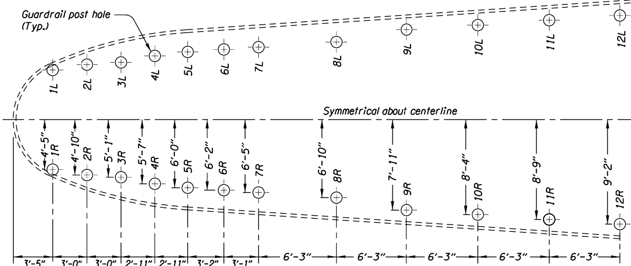
PLAN GUARDRAIL POST LAYOUT - DESIGN 2
