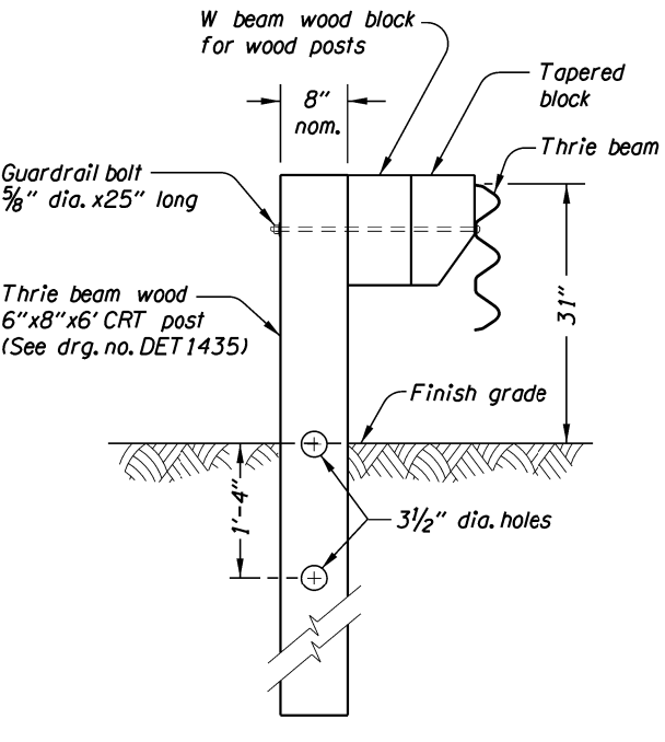
POST 3R TO 8R & 3L TO 8L
