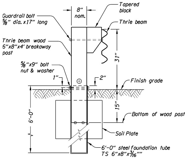
POST 2R & 2L
