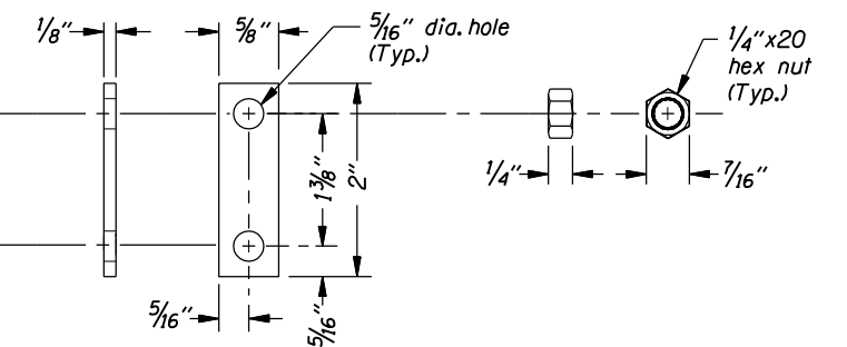
U-BOLT PLATE WASHER
