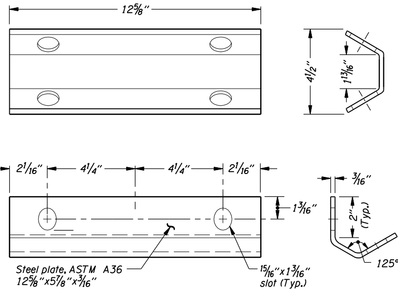
NOSE CABLE ANCHOR PLATE
