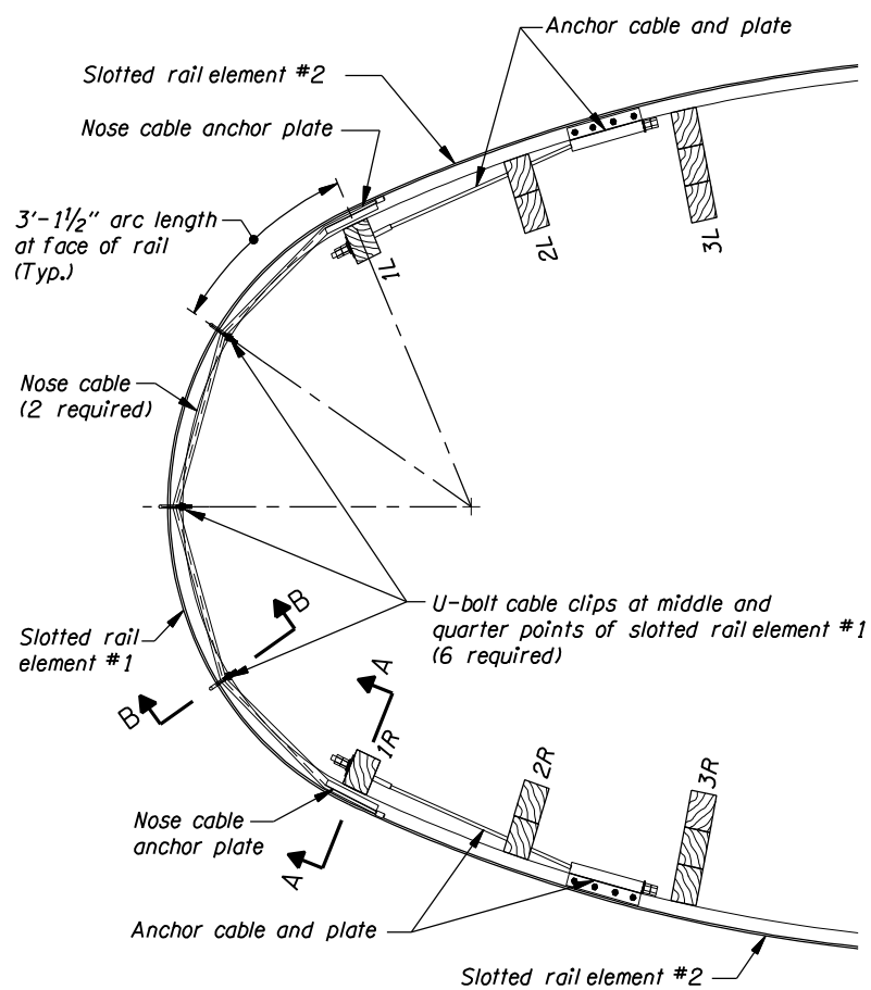
PLAN THRIE BEAM NOSE
