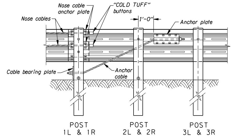
CABLE ANCHOR & BRACKET ASSEMBLY
