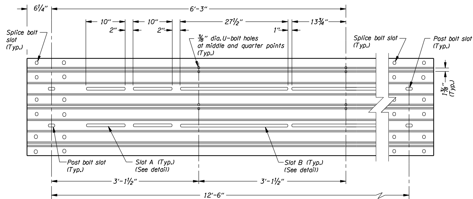
SLOTTED THRIE BEAM RAIL ELEMENT #1 (Rail dimensions shown are before bending to radius shown in plan)
