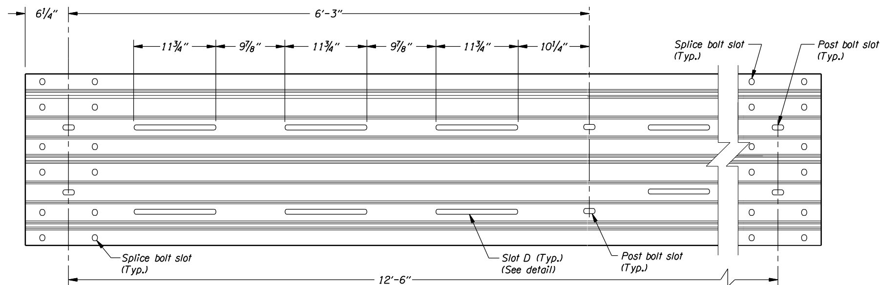
SLOTTED THRIE BEAM RAIL ELEMENT #3 (Rail dimensions shown are before bending to radius shown in plan)
