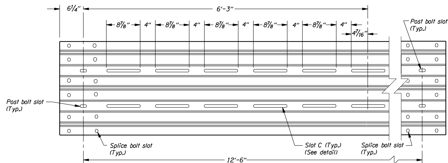
SLOTTED THRIE BEAM RAIL ELEMENT #2 (Rail dimensions shown are before bending to radius shown in plan)
