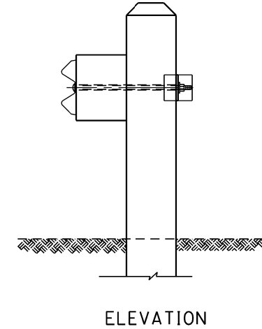
"W" GUARDRAIL RECYCLED PLASTIC PROTECTOR
