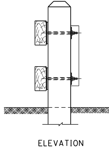
TIMBER GUARDRAIL PVC PROTECTOR
