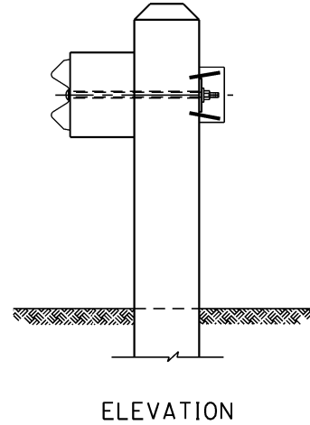
"W" GUARDRAIL PVC PROTECTOR
