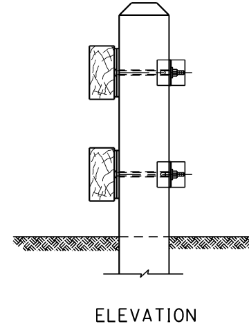
TIMBER GUARDRAIL RECYCLED PLASTIC PROTECTOR
