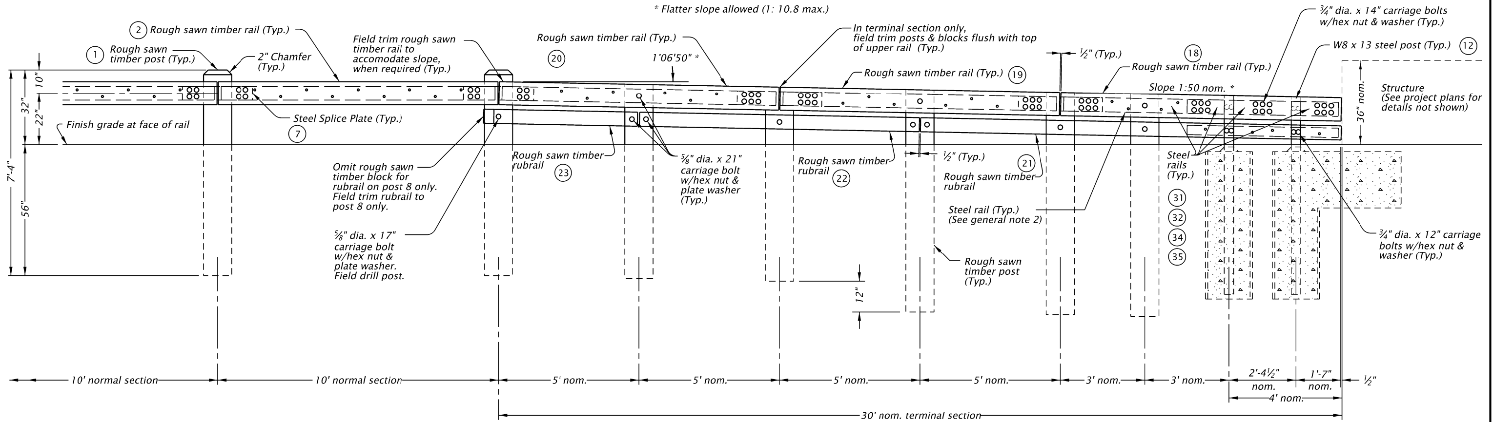
FRONT VIEW
