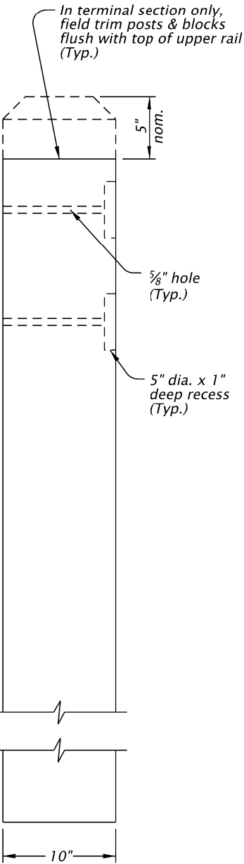
SIDE VIEW
