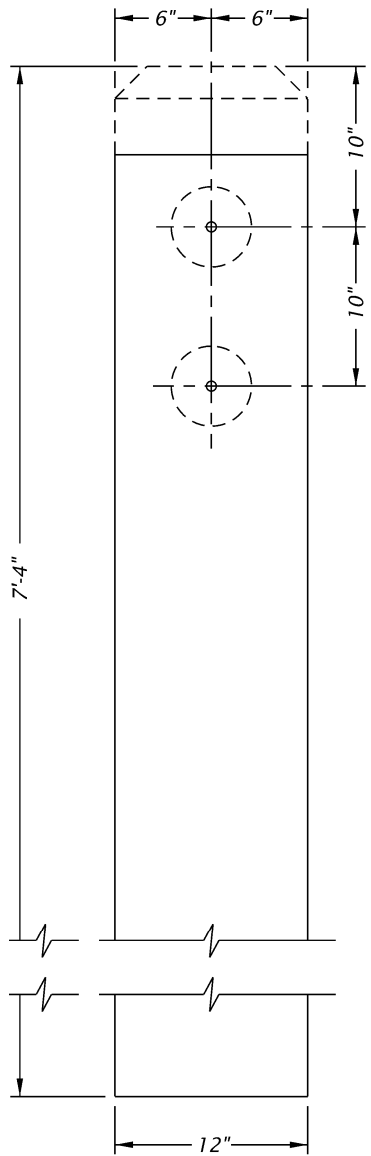
FRONT VIEW
