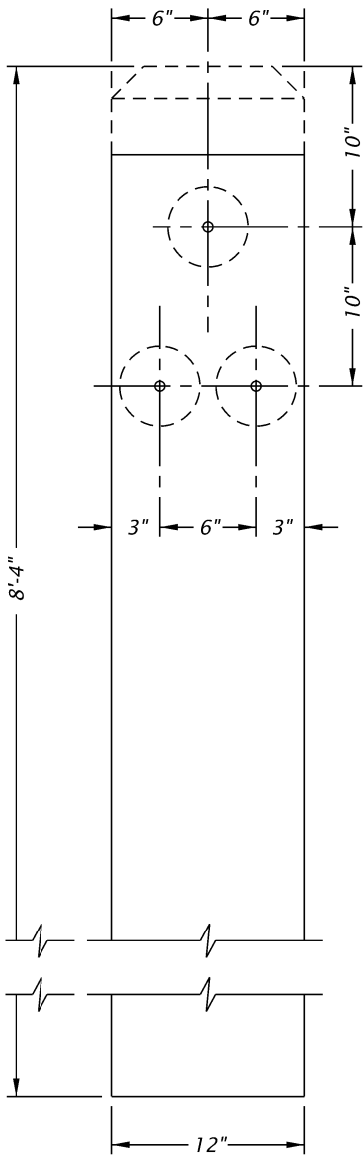
FRONT VIEW
