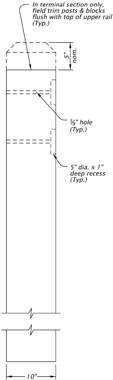
SIDE VIEW
