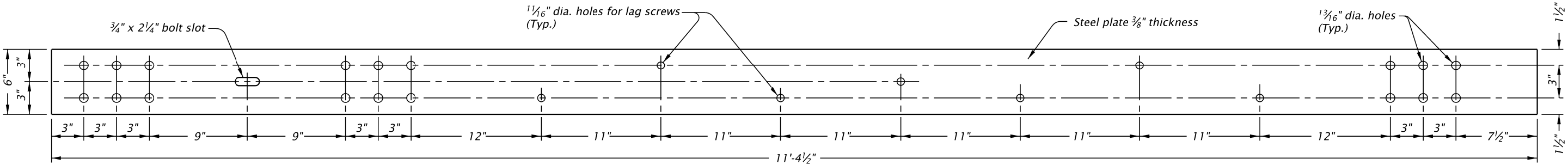
STEEL TRANSITION SECTION (27)
