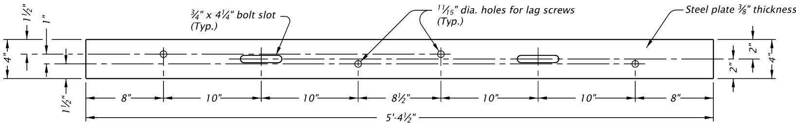
STEEL RUBRAIL TRANSITION SECTION (29)
