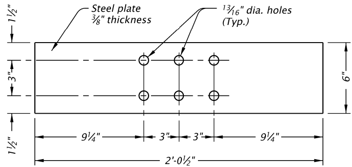
STEEL TERMINAL SECTION (34)
