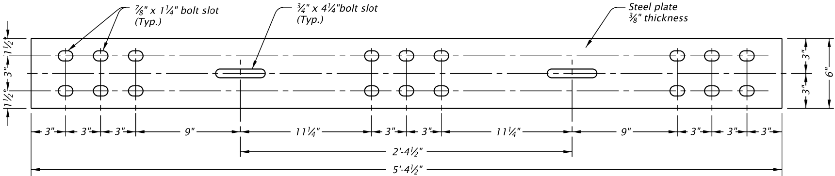
STEEL SPLICE PLATE (31)
