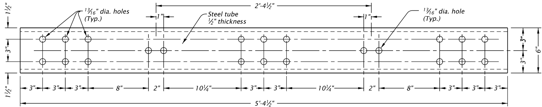
HSS (STEEL TUBE) 6" x 4" x 1/2" (30)
