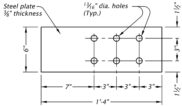
STEEL TERMINAL SECTION (35)
