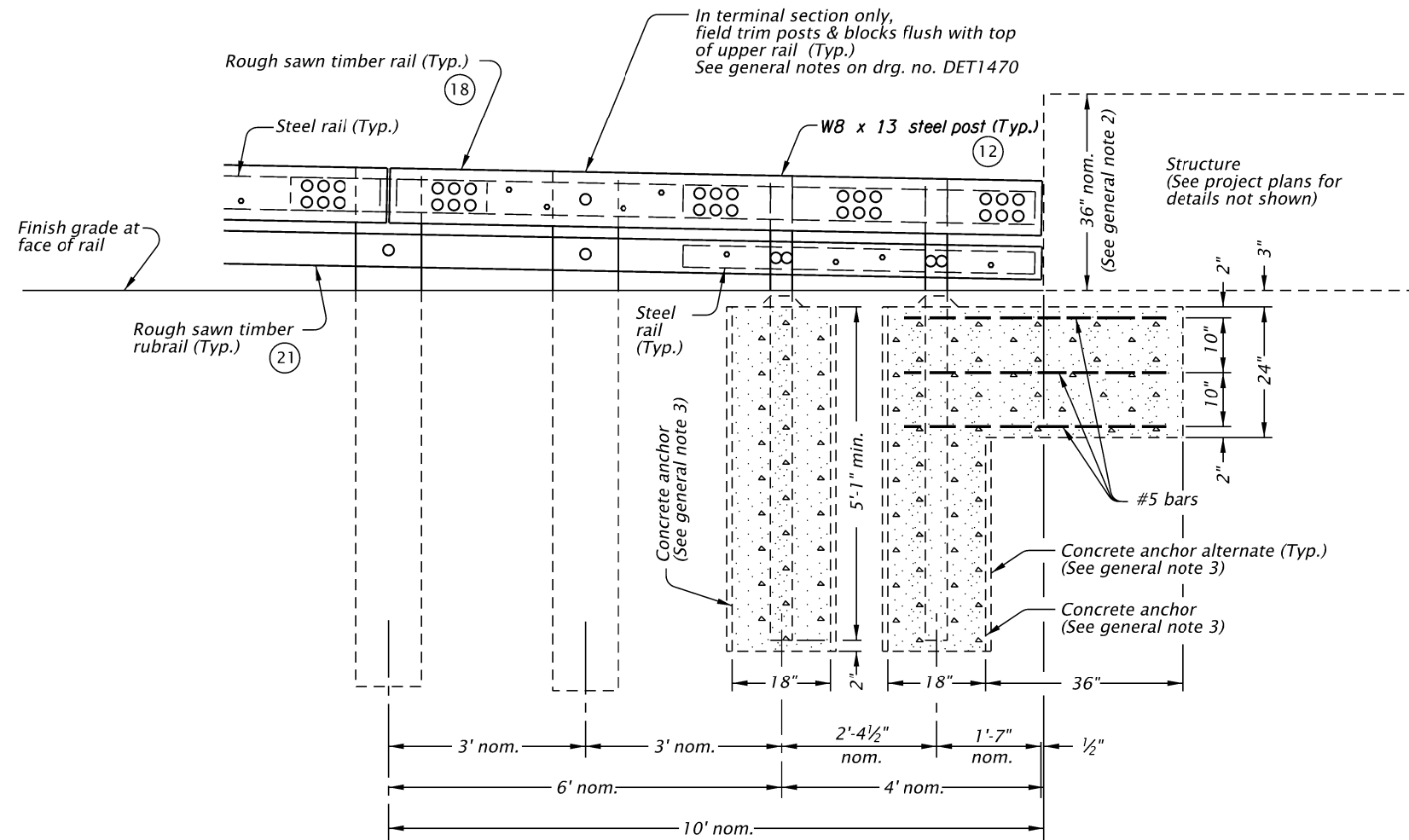
FRONT VIEW
