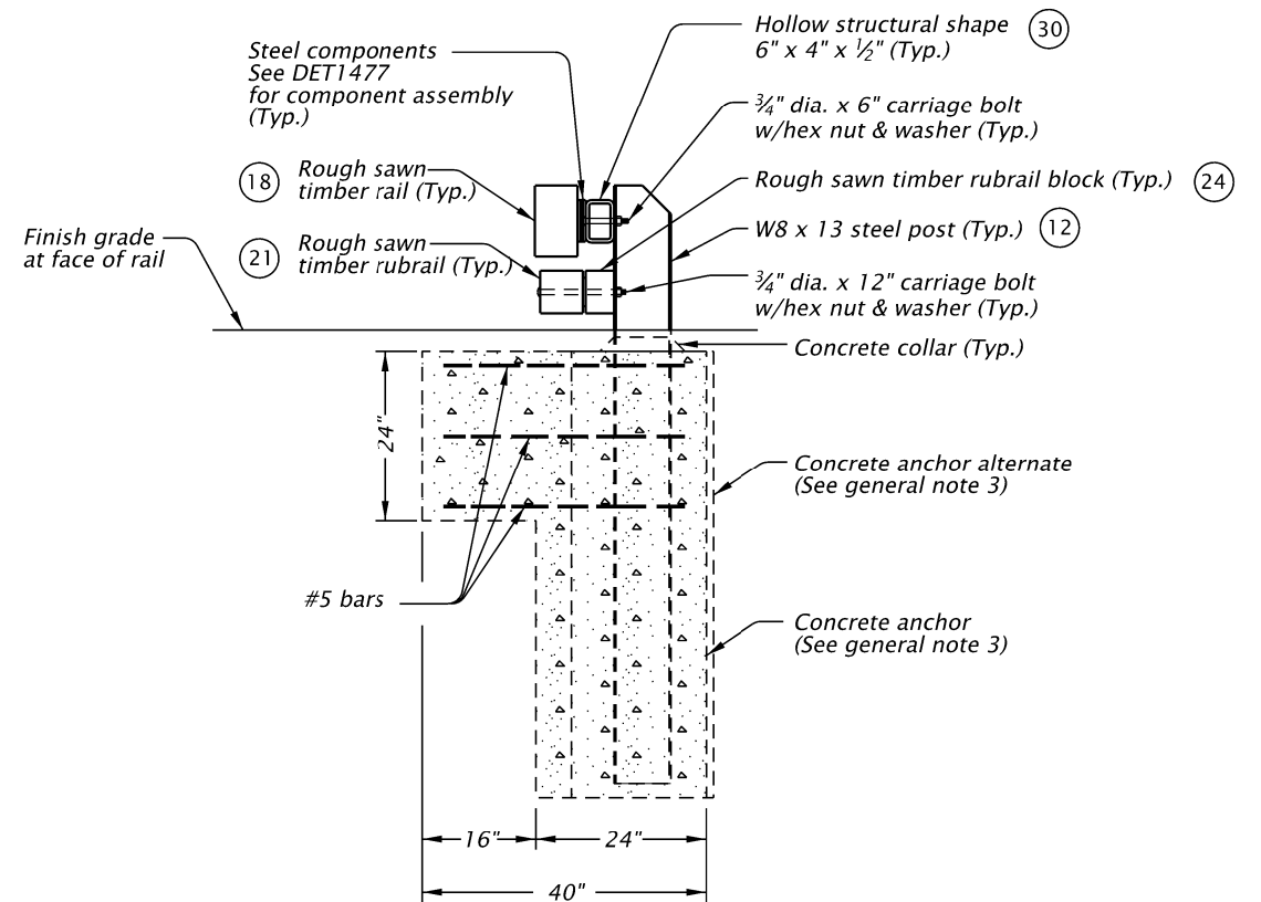
SIDE VIEW
