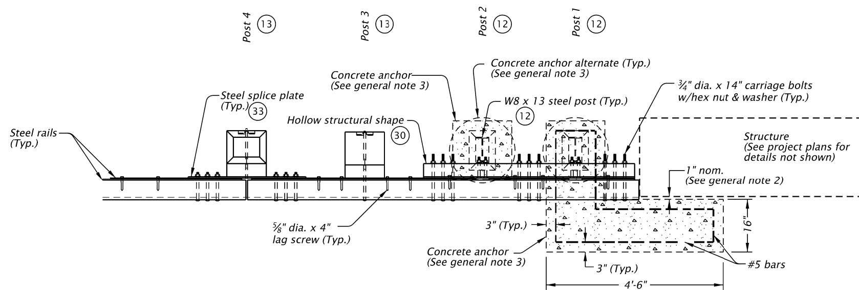
TOP VIEW
