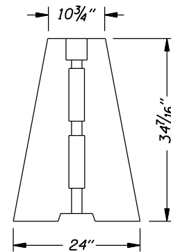
SECTION C-C
