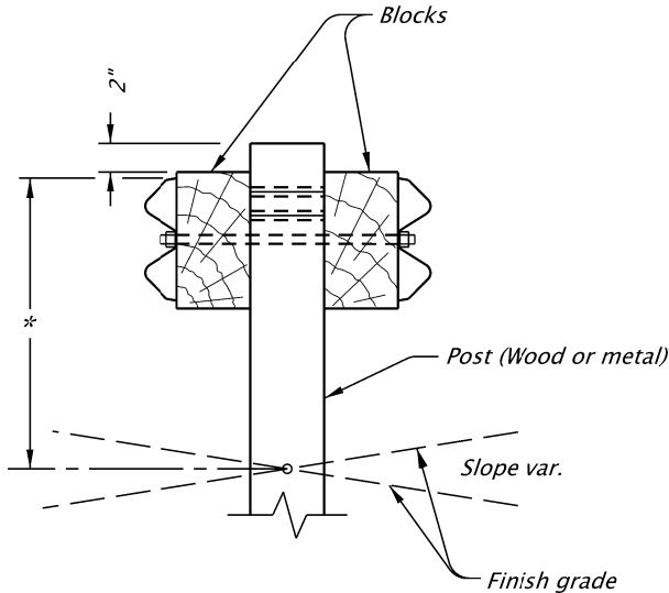
SECTION MEDIAN RAIL (No Rub Rail)
