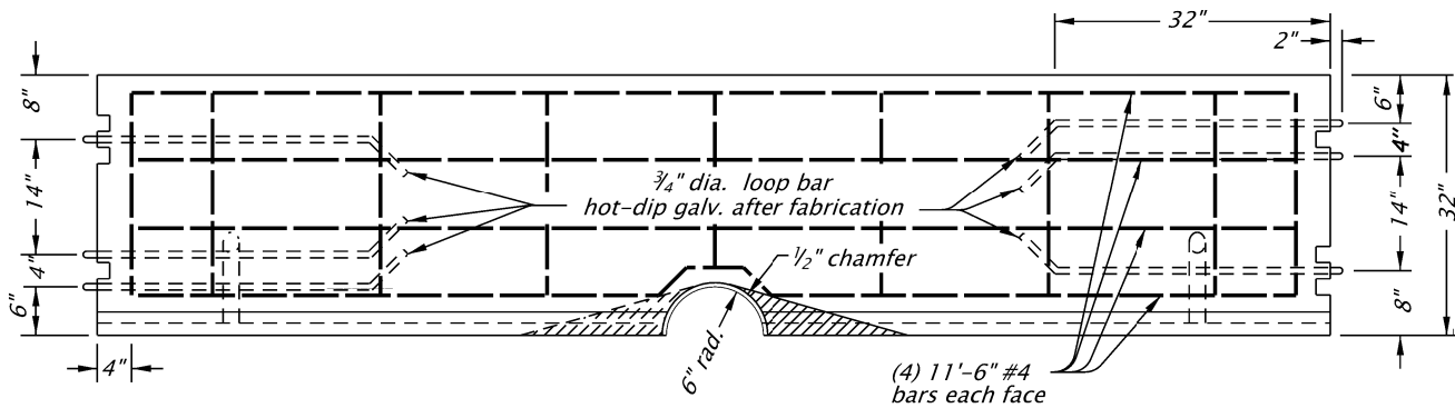
MEDIAN BARRIER
