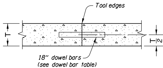
SECTION A-A CONSTRUCTION JOINT
