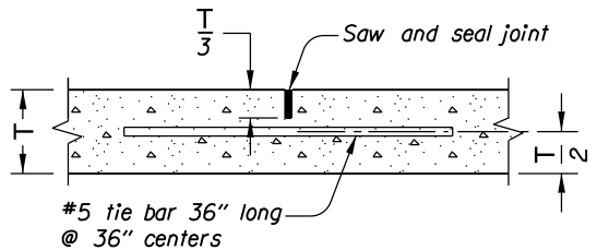
WEAKENED PLANE JOINT
