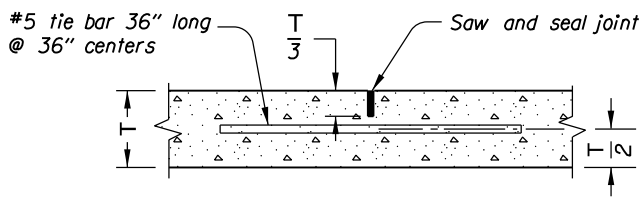
WEAKENED PLANE JOINT
