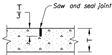
SECTION B-B CONTRACTION JOINT
