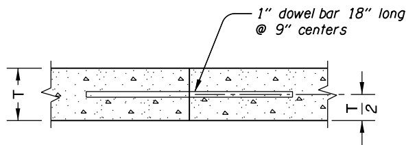
SECTION A-A CONSTRUCTION JOINT
