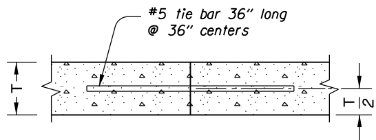
CONTACT JOINT
