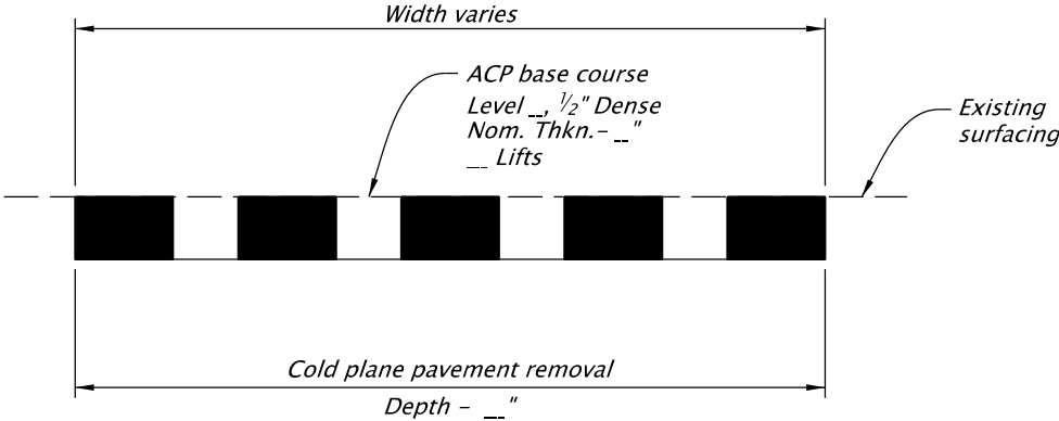
PARTIAL DEPTH ACPR x" ASPHALT CONCRETE PAVEMENT REPAIR
