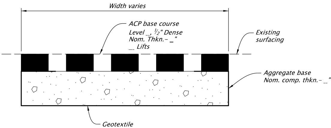
FULL DEPTH ACPR x" ASPHALT CONCRETE PAVEMENT REPAIR
