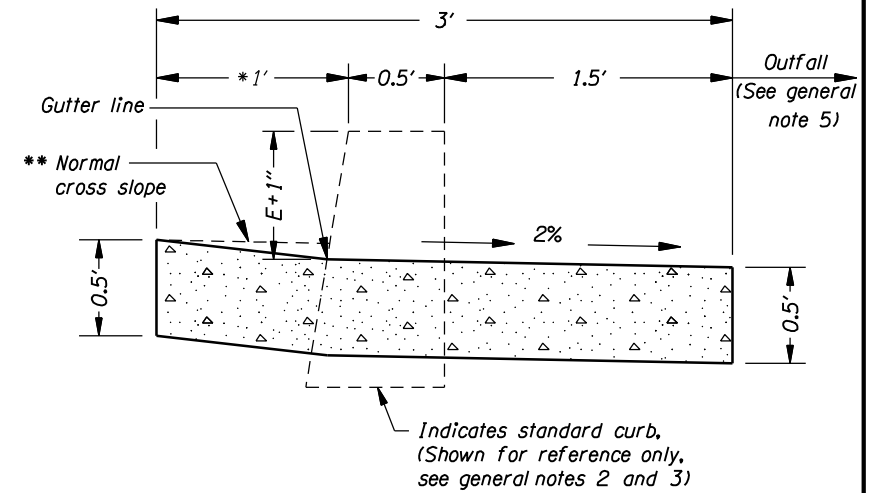
SEC. B-B
