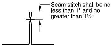
"FLAT" OR "PRAYER" SEAM SSa-1
