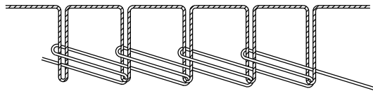
STITCH TYPE 401
