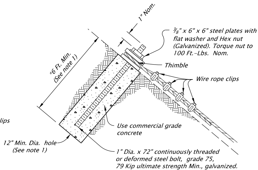
STEEL BOLT ANCHOR TYPE
