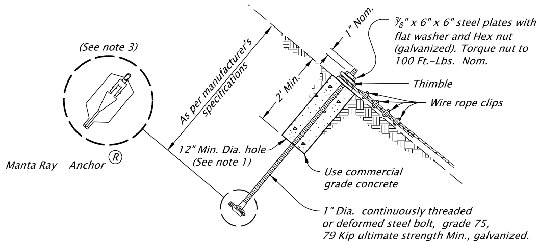
MANTA RAY ® TYPE
