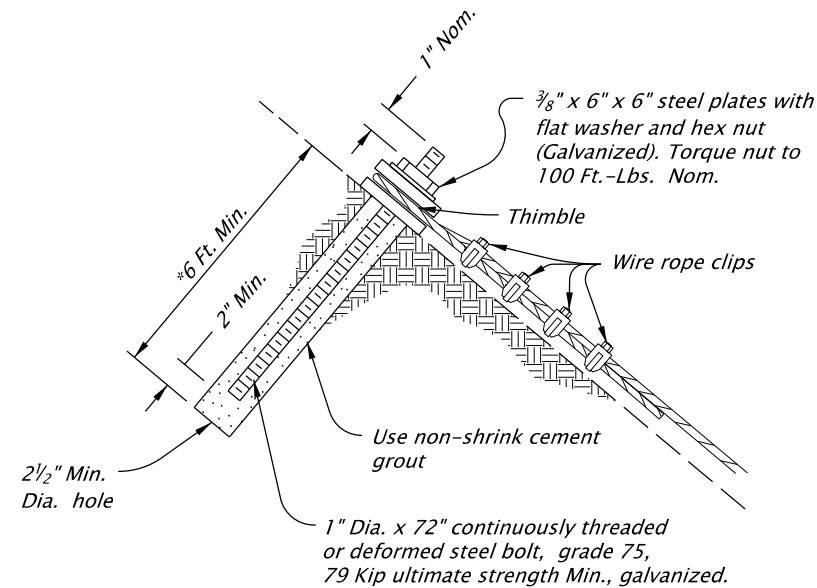
STEEL BOLT ANCHOR TYPE
