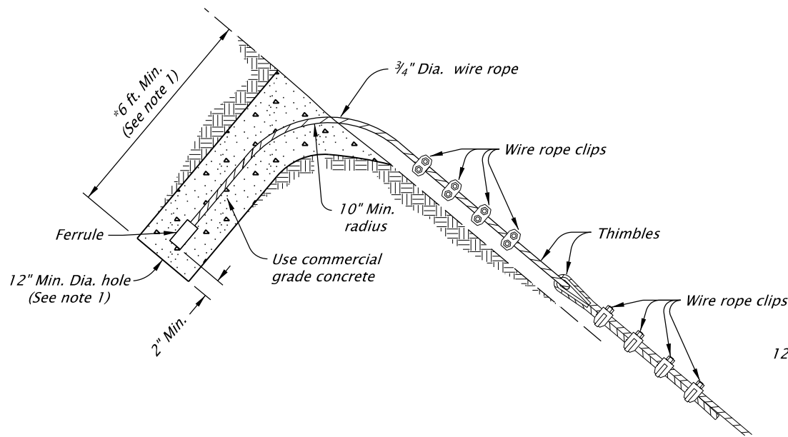
3/4" WIRE ROPE TYPE
