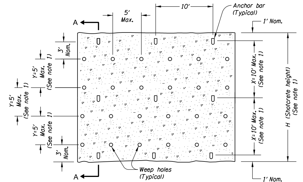
SPACING OF ANCHOR BARS &amp; DRAIN PIPES
