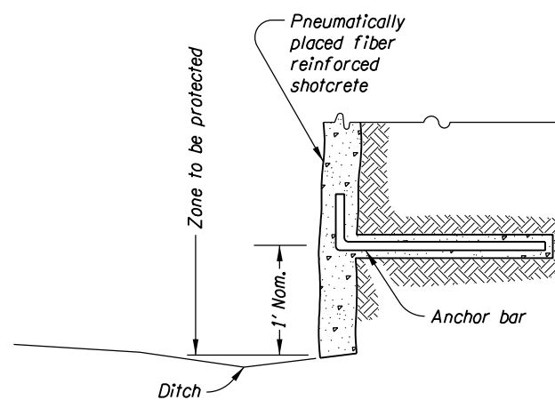
SHOTCRETE AT TOE OF SLOPE
