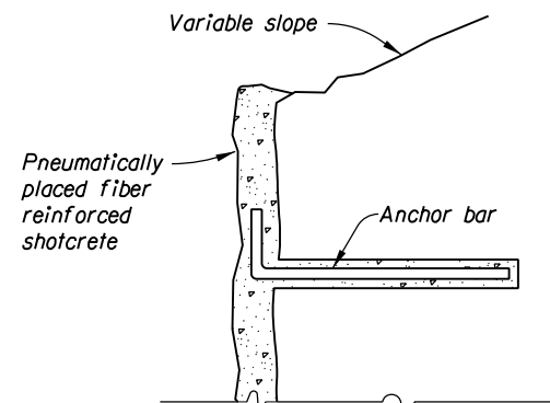
SHOTCRETE AT TOP OF CUT SLOPE
