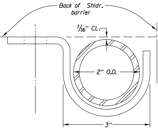
ALTERNATE POST & CLAMP
