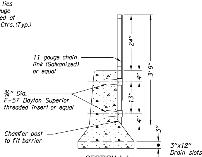
Precast Conc. Shldr. barrier (pin & loop) (For details not shown, see Drg. No. RD500)
