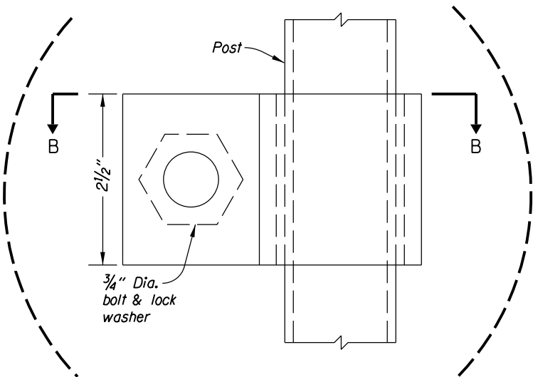
POST CLAMP DETAIL "A"
