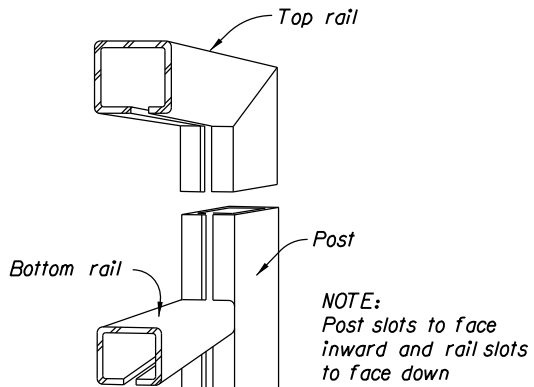
POST & RAIL ASSEMBLY
