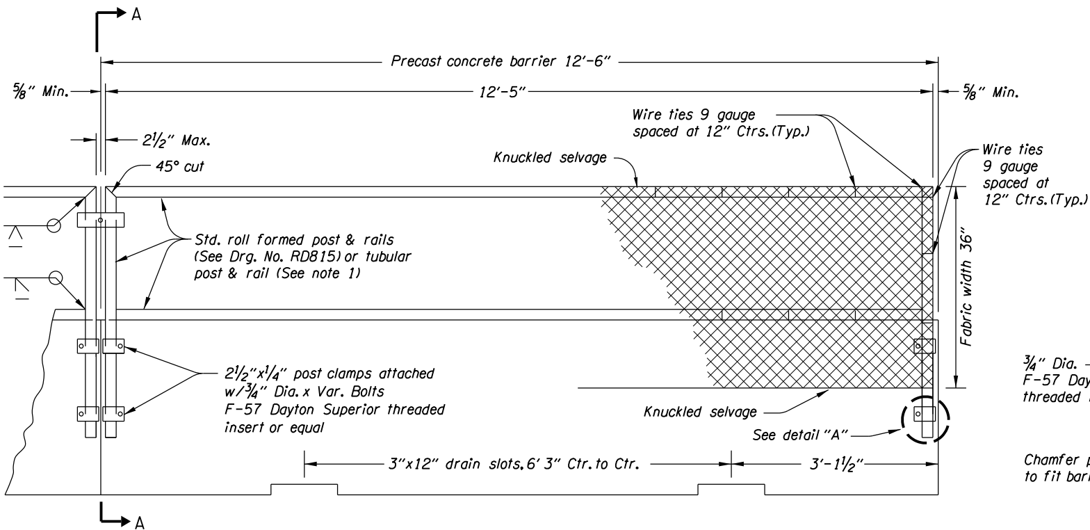
ROCK PROTECTION SCREEN ATTACHMENT
