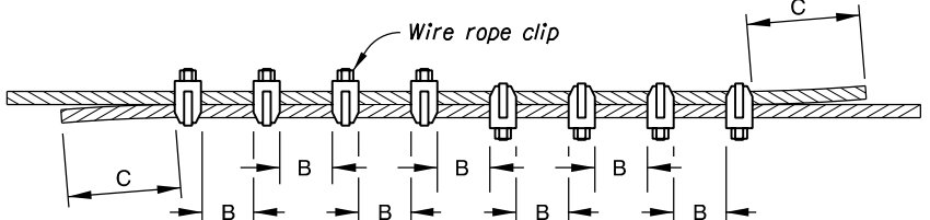
DISTANCES B, C, AND TORQUE TO COMPLY WITH MANUFACTURER'S SPECIFICATIONS
