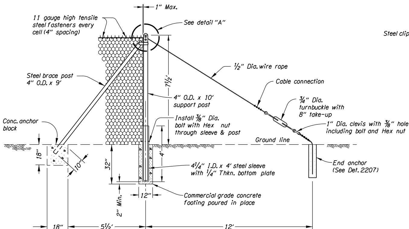
SUPPORT POST & END ANCHORAGE
