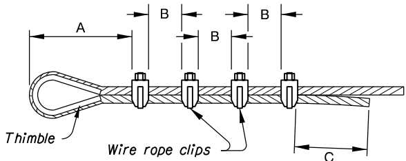
DISTANCES A, B, C, AND TORQUE TO COMPLY WITH MANUFACTURER'S SPECIFICATIONS
