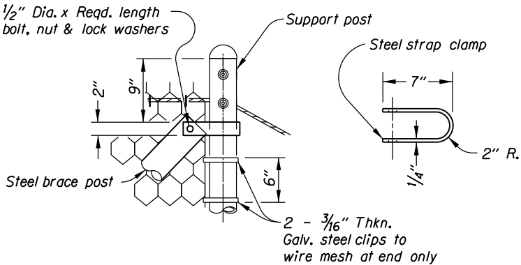
POST BRACE - STRAP CLAMP DETAIL
