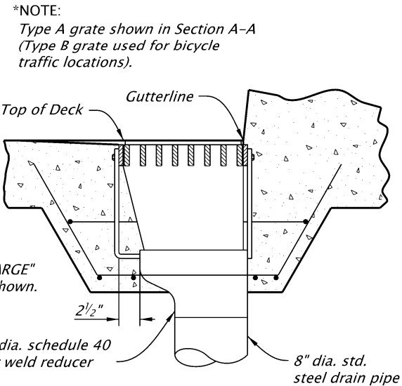
SECTION A-A - OFFSET DISCHARGE
