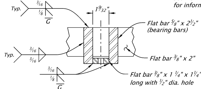
SECTION B-B - Type A Grate
