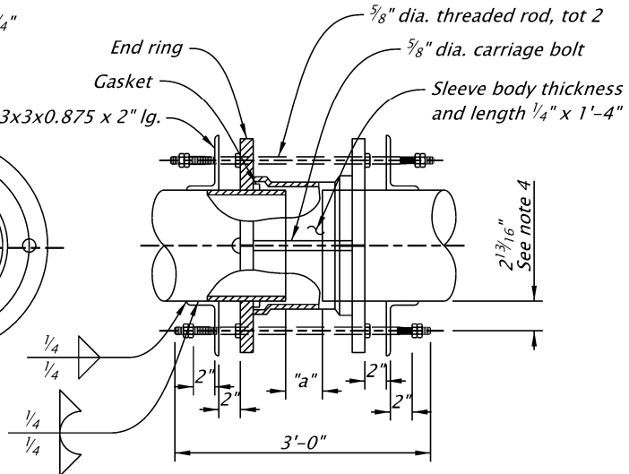
EXPANSION COUPLING
