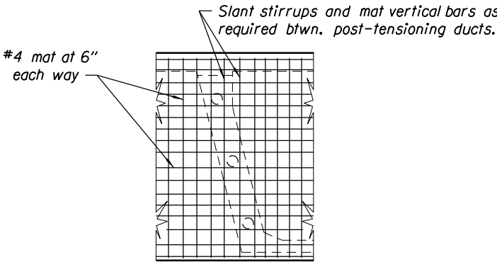
CONTINUOUS MAT ELEVATION BEAM "E"
