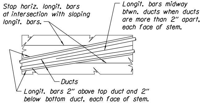
LONGITUDINAL STEM REINFORCING AT DUCT PART ELEVATION OF GIRDER STEM
