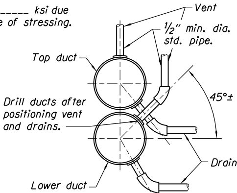
GROUT VENT DETAIL FOR HIGH POINT VENTS AND LOW POINT DRAINS
