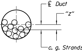
TENDON LIMITATION DETAIL (CAST-IN-PLACE BOX)
