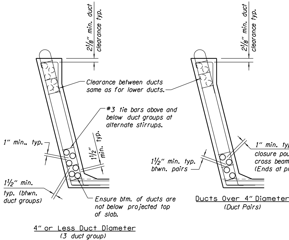
TENDON LIMITATION DETAILS PRECAST BOXES
