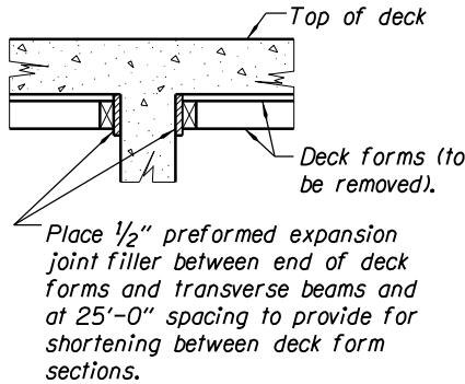
TENDON FORM DETAIL
