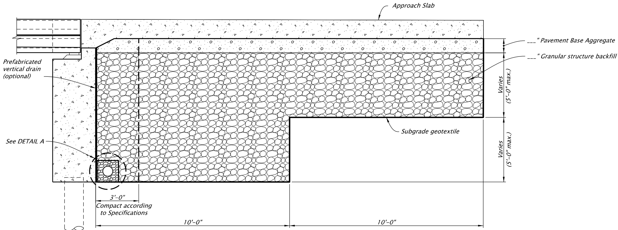
APPROACH SLAB SECTION Scale: No Scale
