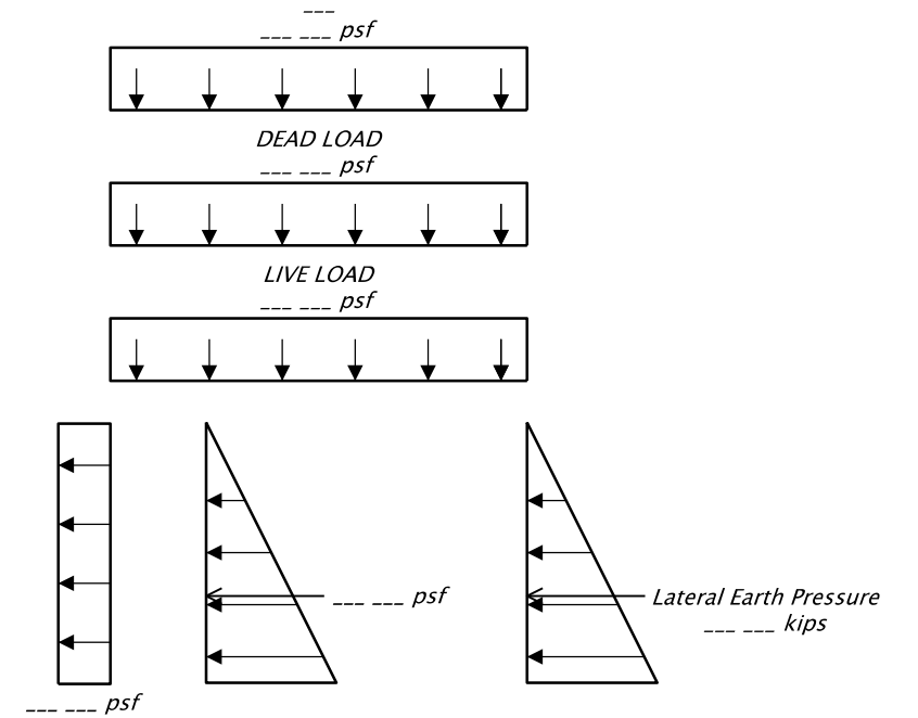
LOAD DIAGRAMS Not to Scale
