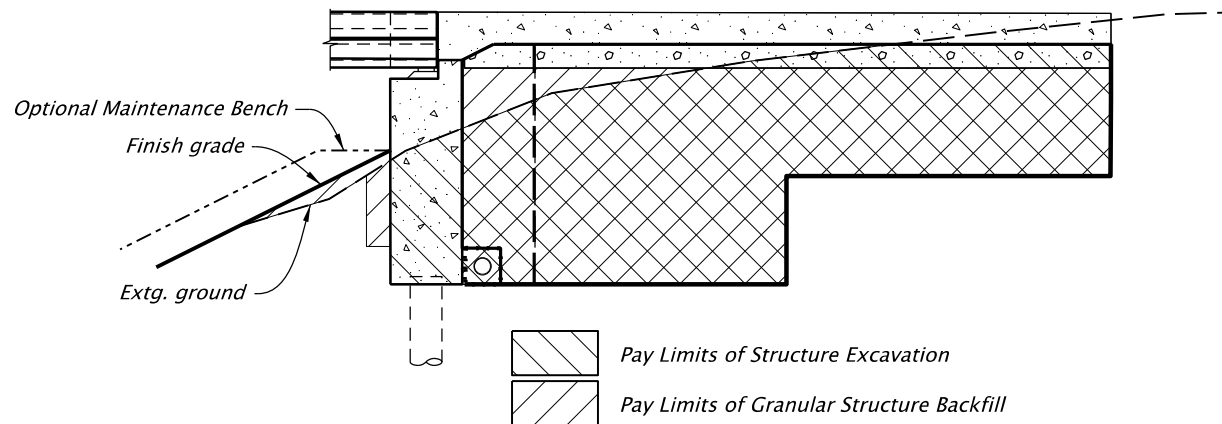
STRUCTURE EXCAVATION AND BACKFILL PAY LIMITS Scale: No Scale
