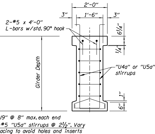
BULB-I END BLOCK SECTION
