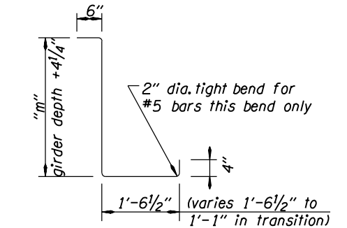
BAR "U4a" or "U5a"
