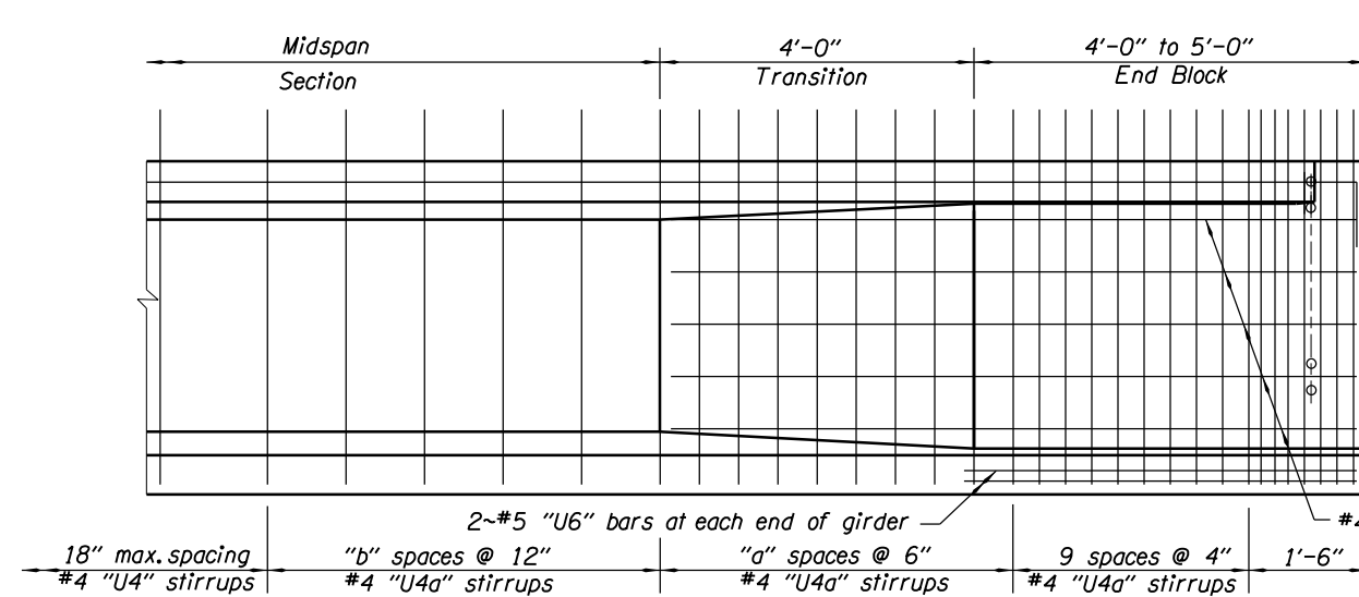
BULB-I END BLOCK SIDE ELEVATION
