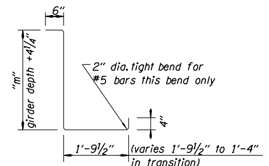
BAR "U4a" or "U5a" (For BT90 AND BT96 Only)
