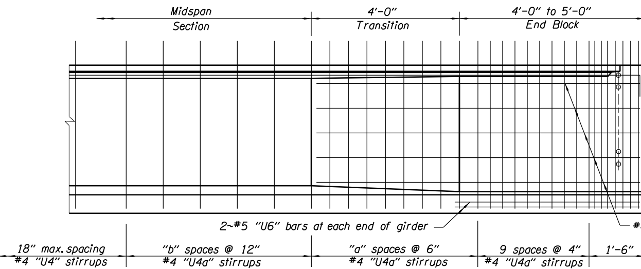
BULB-T END BLOCK SIDE ELEVATION
