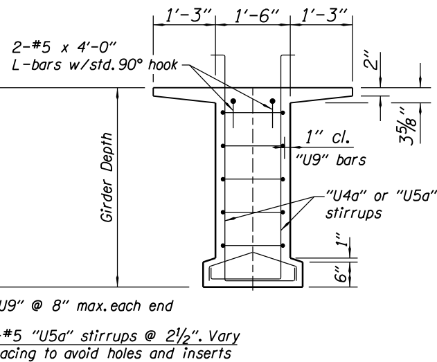
BULB-T END BLOCK SECTION
