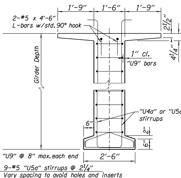
BT90 AND BT96 END BLOCK SECTION
