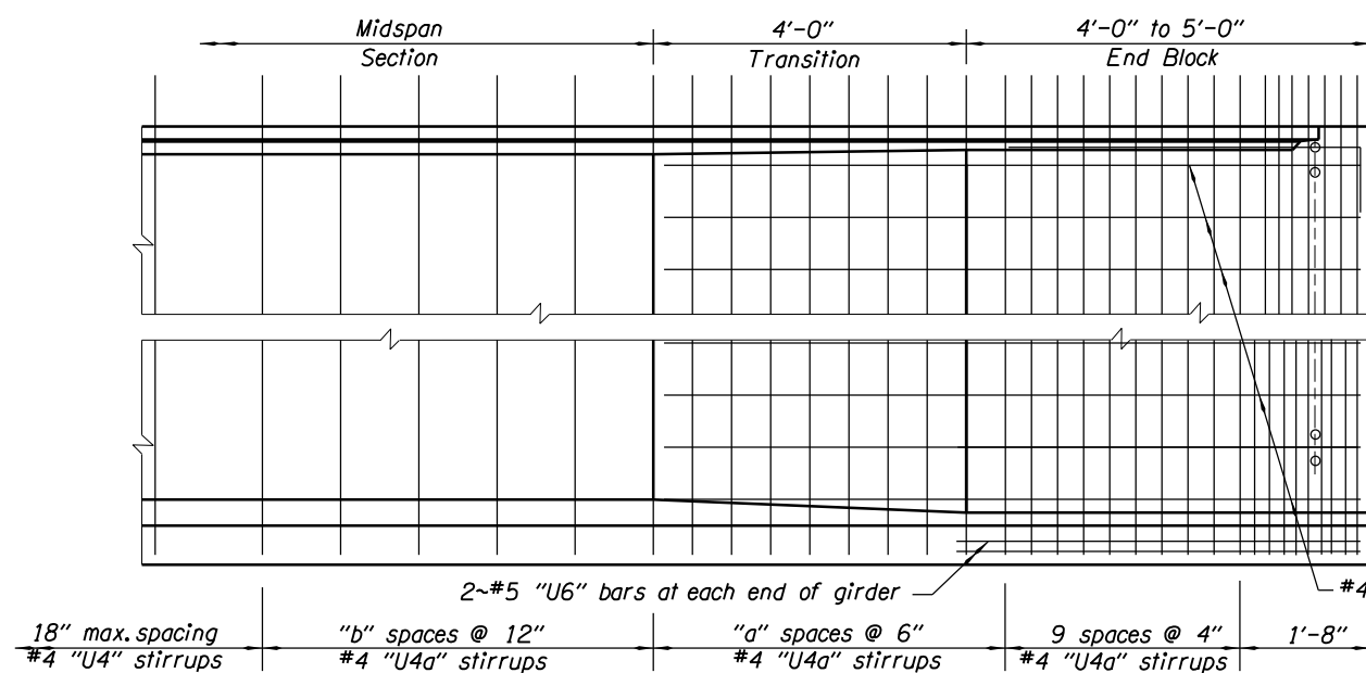
BT90 AND BT96 END BLOCK SIDE ELEVATION
