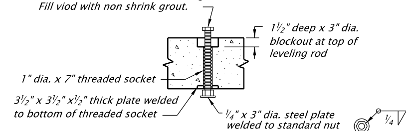
LEVELING ROD DETAIL
