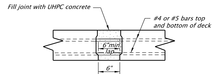
SECTION B-B TRANSVERSE JOINT DETAIL
