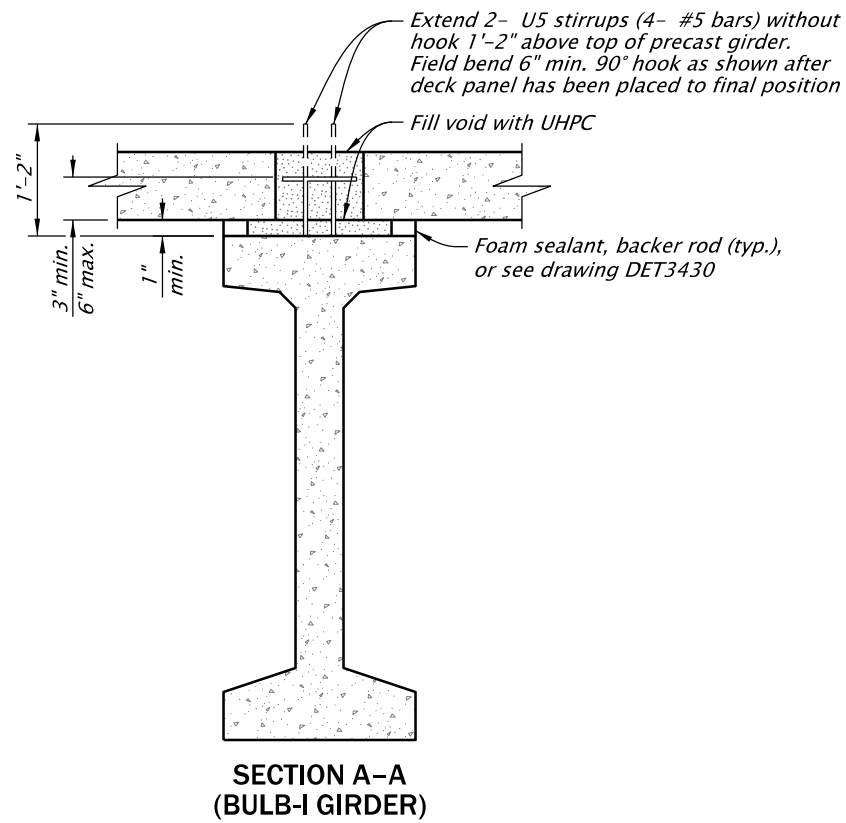
SHEAR BLOCKOUT FOR CONCRETE GIRDERS Scale: 1/2"=1'-0"
