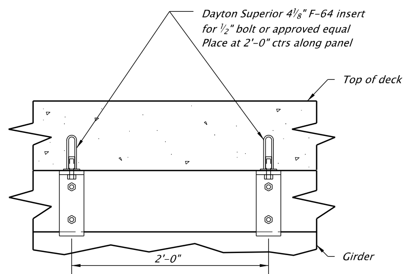
BRACKET LAYOUT
