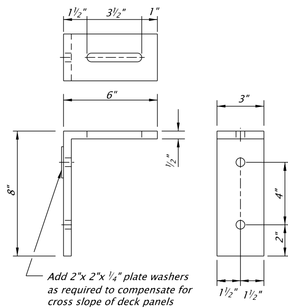
STEEL BRACKET DETAIL
