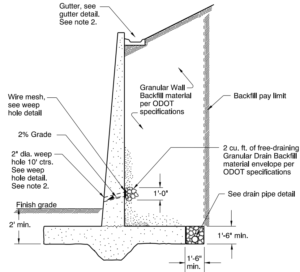
DRAINAGE (Normal condition)
