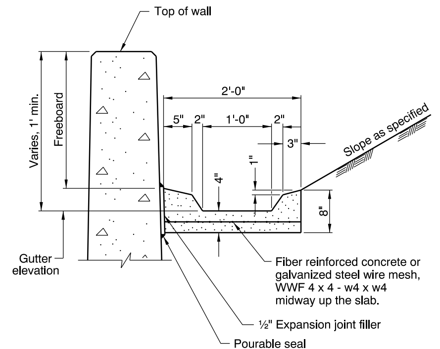
TYPICAL GUTTER and FREEBOARD DETAIL (See note 2)
