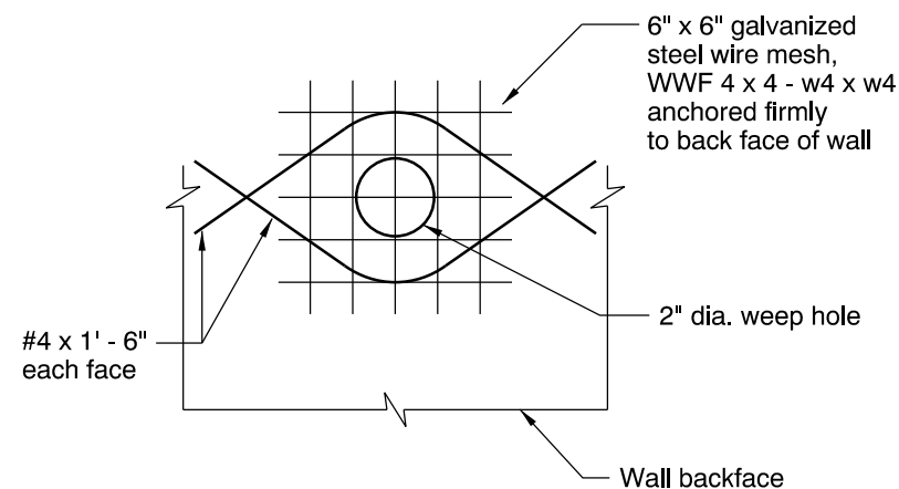
WEEP HOLE DETAIL (See note 2)
