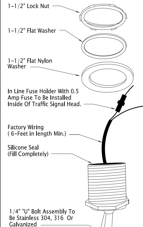
SIGNAL HOUSING DETAIL (BOTTOM SECTION)
