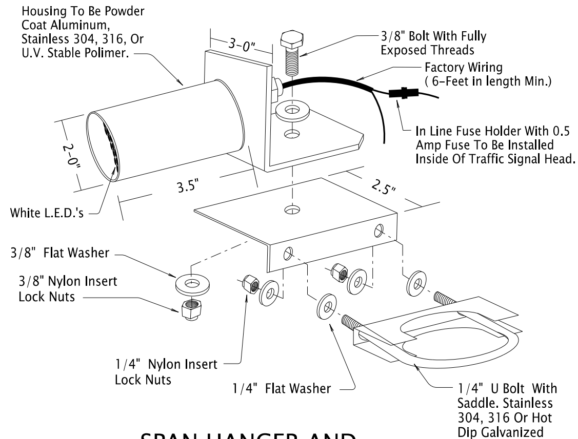
SPAN HANGER AND GUSSETED TUBE MOUNT
