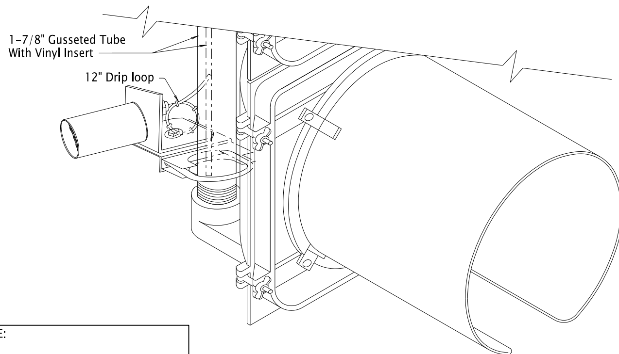
GUSSETED TUBE MOUNTING DETAIL
