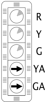
TYPE 5 Protected / Permitted Right Turn
