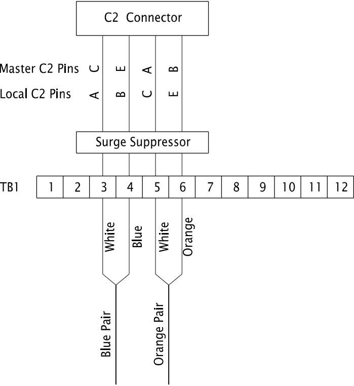
TB1 WIRING DIAGRAM
