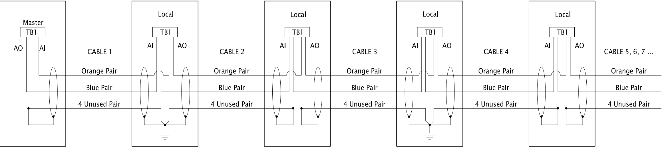
TYPICAL 6 PAIR INTERCONNECT WIRING DIAGRAM
