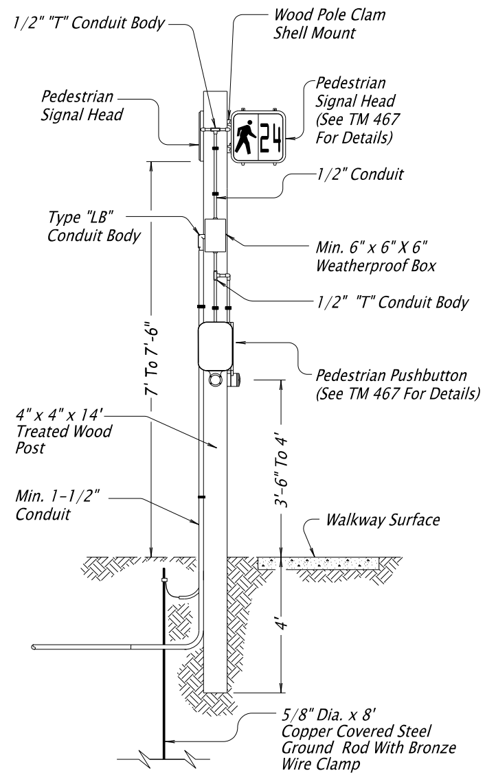
TYPICAL PEDESTRIAN INSTALLATION ON WOOD POST (UNDERGROUND CONDUIT)
