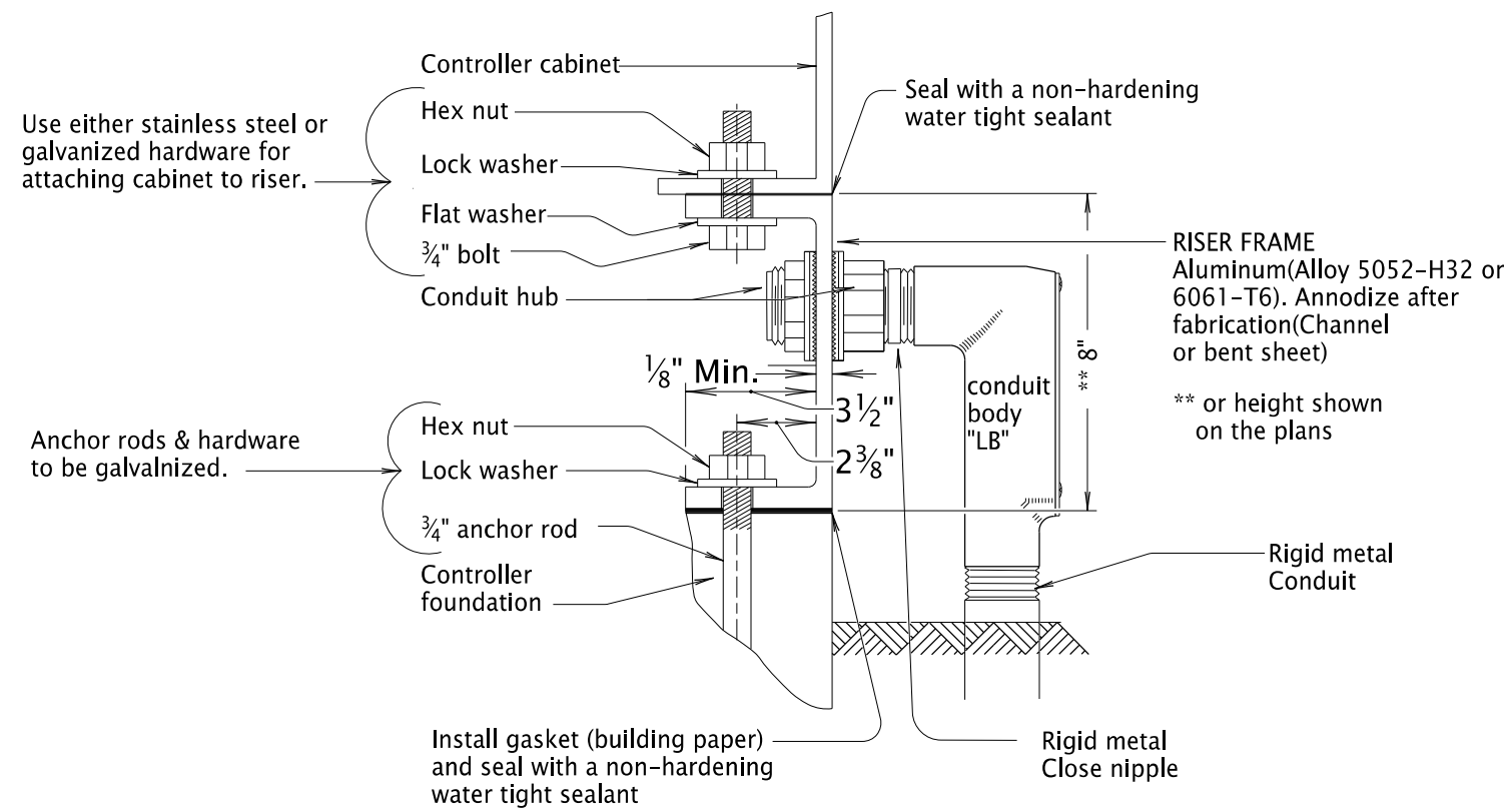
RISER FRAME CONNECTION DETAIL 332, 334, AND 340 CABINET RISER FRAME
