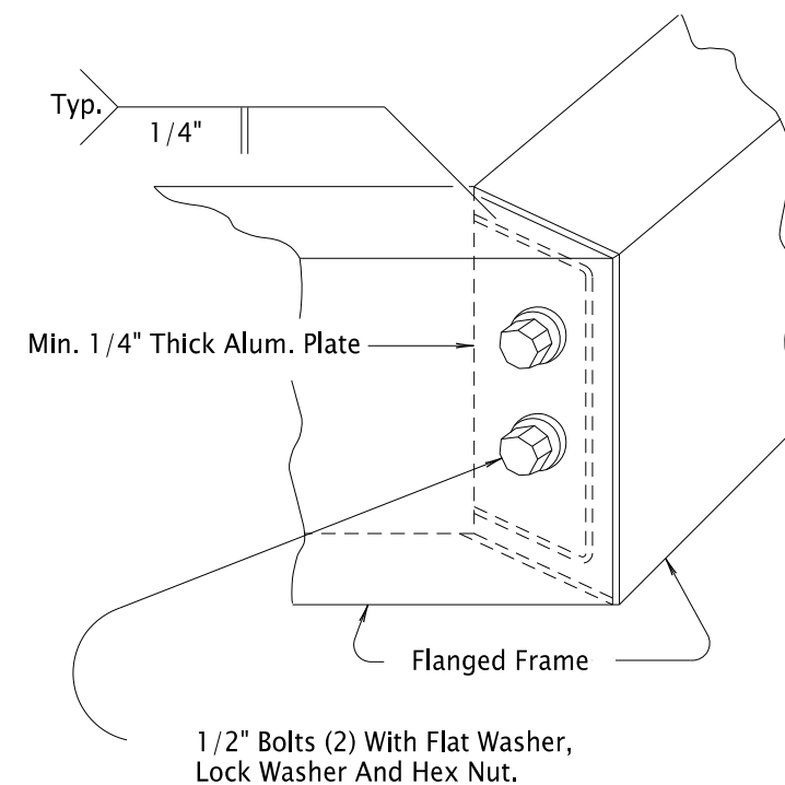
BOLTED RISER FRAME DETAIL
