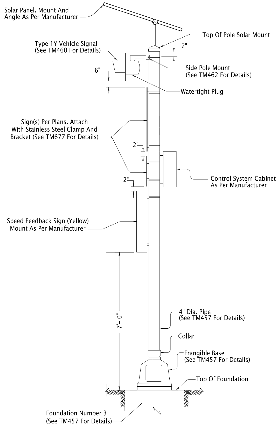
24 / 7 FLASHING BEACON ASSEMBLY WITH SPEED FEEDBACK SIGN (Use Green Sheet Listed Items Only)
