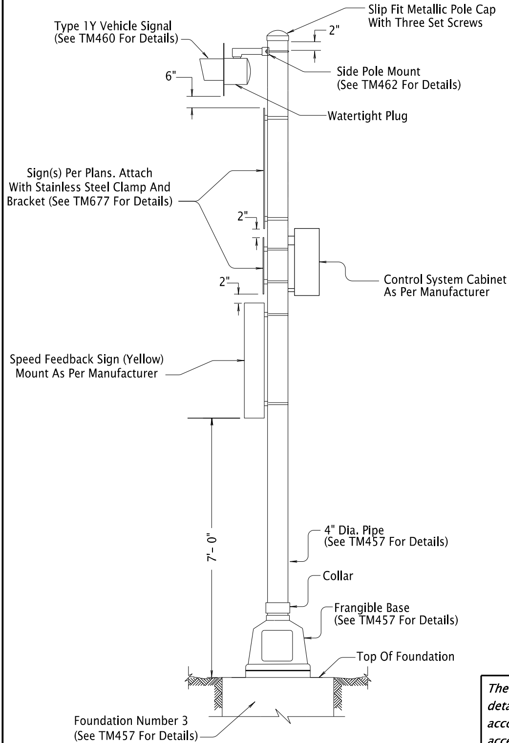
24 / 7 FLASHING BEACON ASSEMBLY WITH SPEED FEEDBACK SIGN (Use Green Sheet Listed Items Only)
