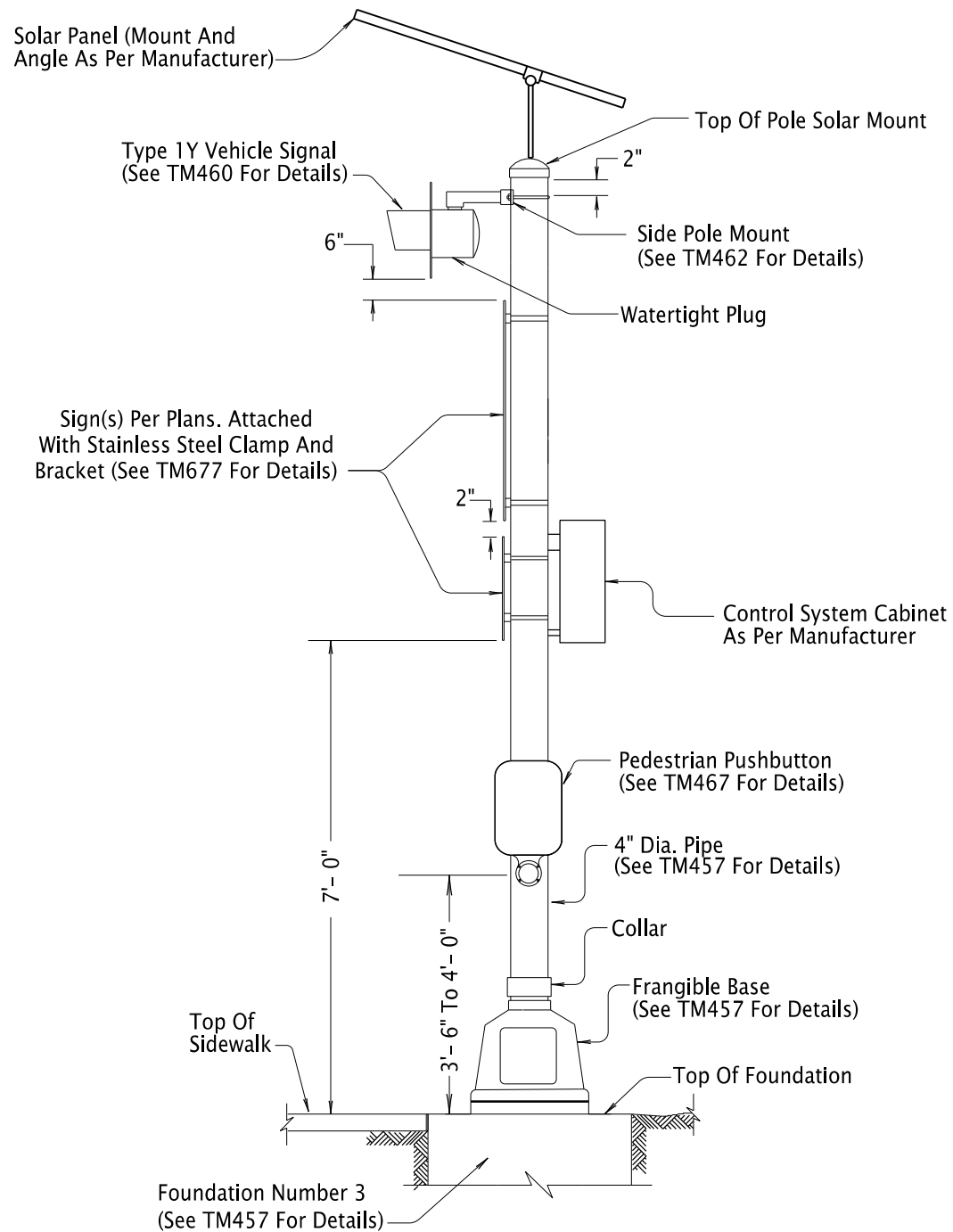
ACTUATED FLASHING BEACON ASSEMBLY – PED (Use Green Sheet Listed Items Only)
