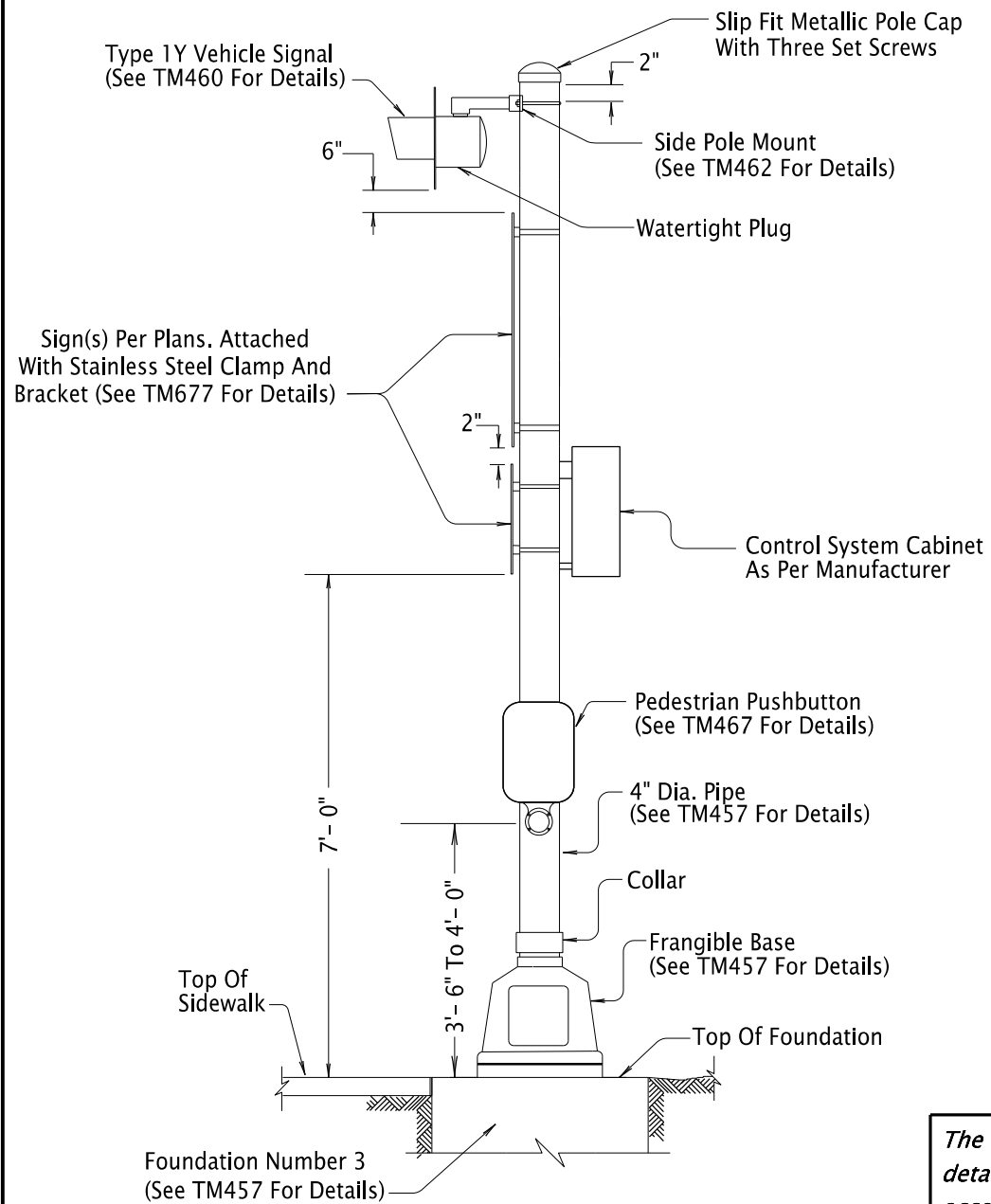
ACTUATED FLASHING BEACON ASSEMBLY – PED (Use Green Sheet Listed Items Only)
