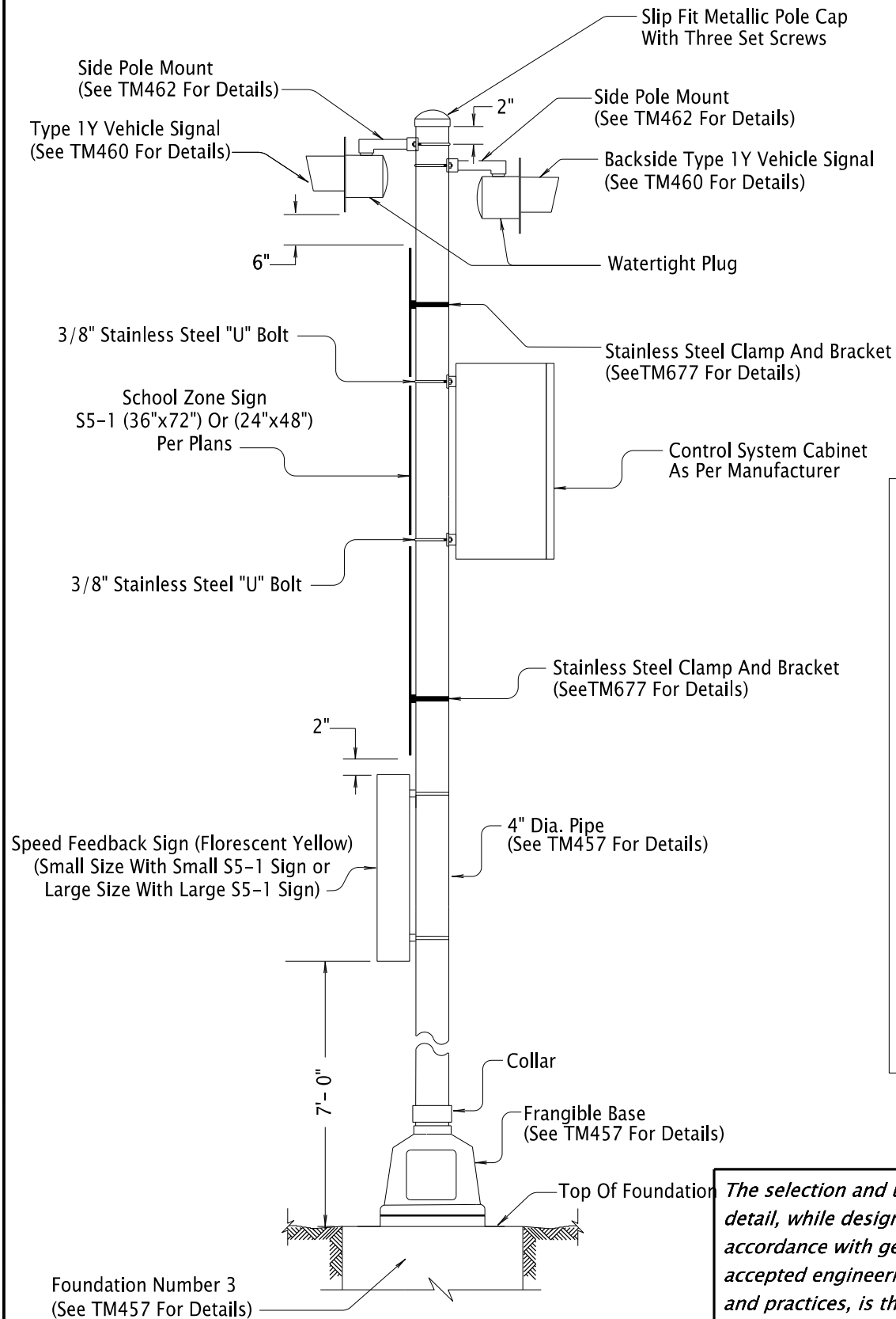
ACTUATED FLASHING BEACON ASSEMBLY: SCHOOL + SPEED FEEDBACK (Use Green Sheet Listed Items Only)
