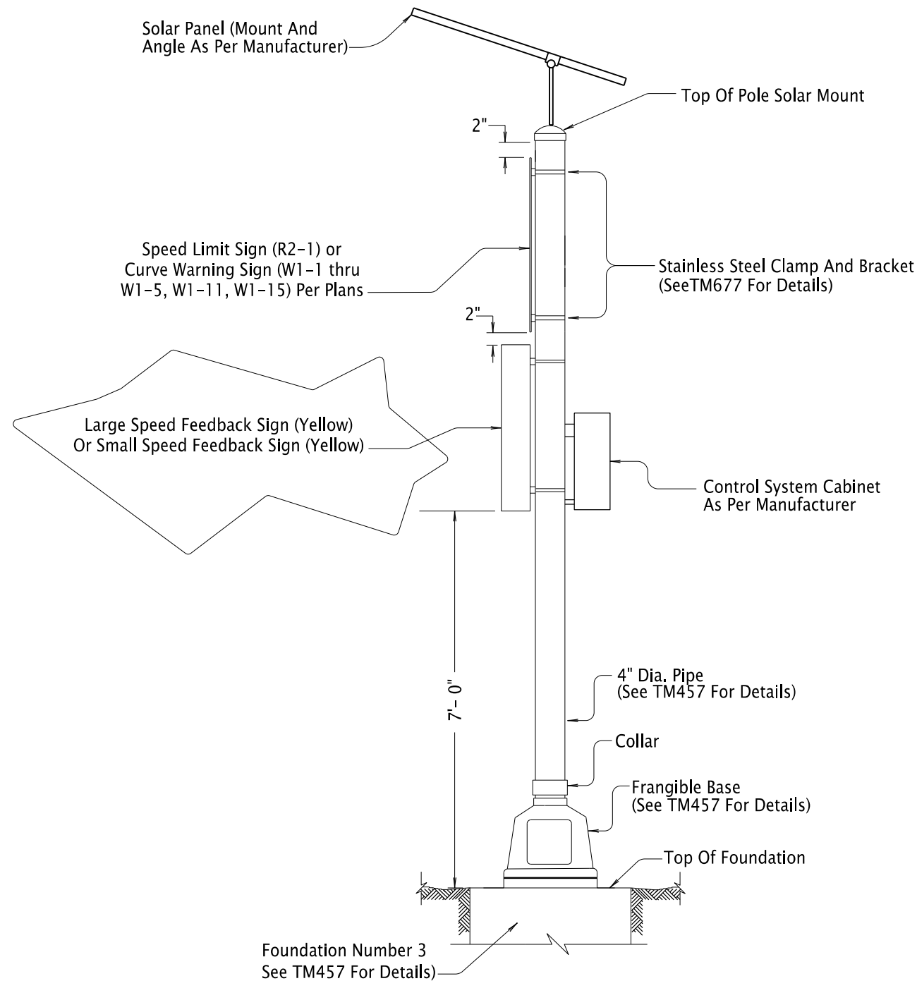
UNINTEGRATED SPEED FEEDBACK ASSEMBLY (Use Green Sheet Listed Items Only)
