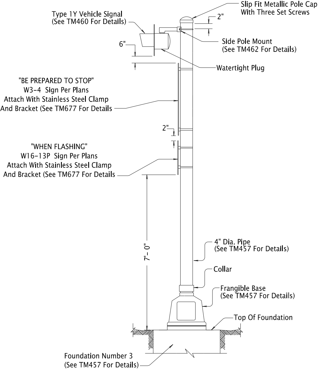
FLASHING BEACON ASSEMBLY FOR SIGN W3-4 & W16-13P SIGNS
