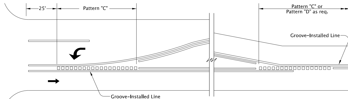
LEFT TURN LANE CENTERLINE RUMBLE STRIP TRANSITION
