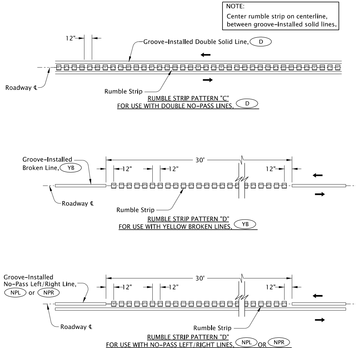
RUMBLE STRIP PATTERNS "C" & "D" (NO MEDIAN INSTALLATION)
