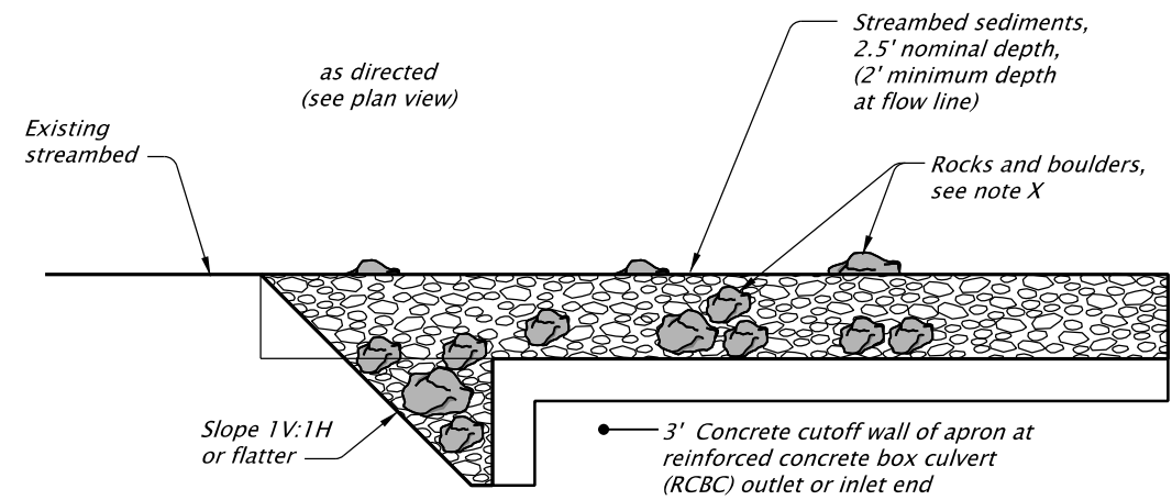
EXISTING STREAMBED TRANSITION PROFILE NOT TO SCALE
