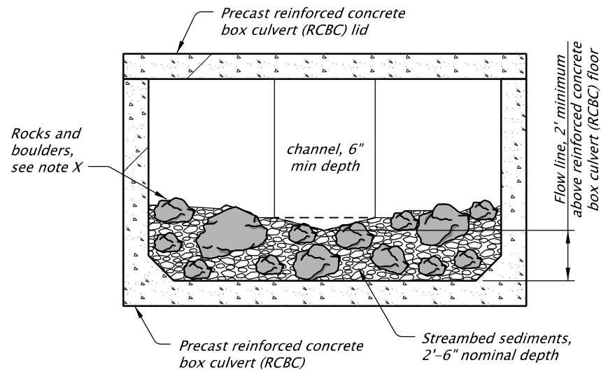
STREAMBED SECTION IN CULVERT NOT TO SCALE
