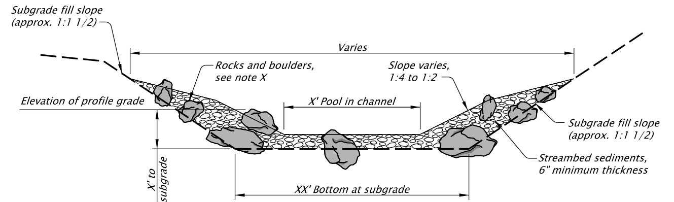
SECTION AT POOLS
