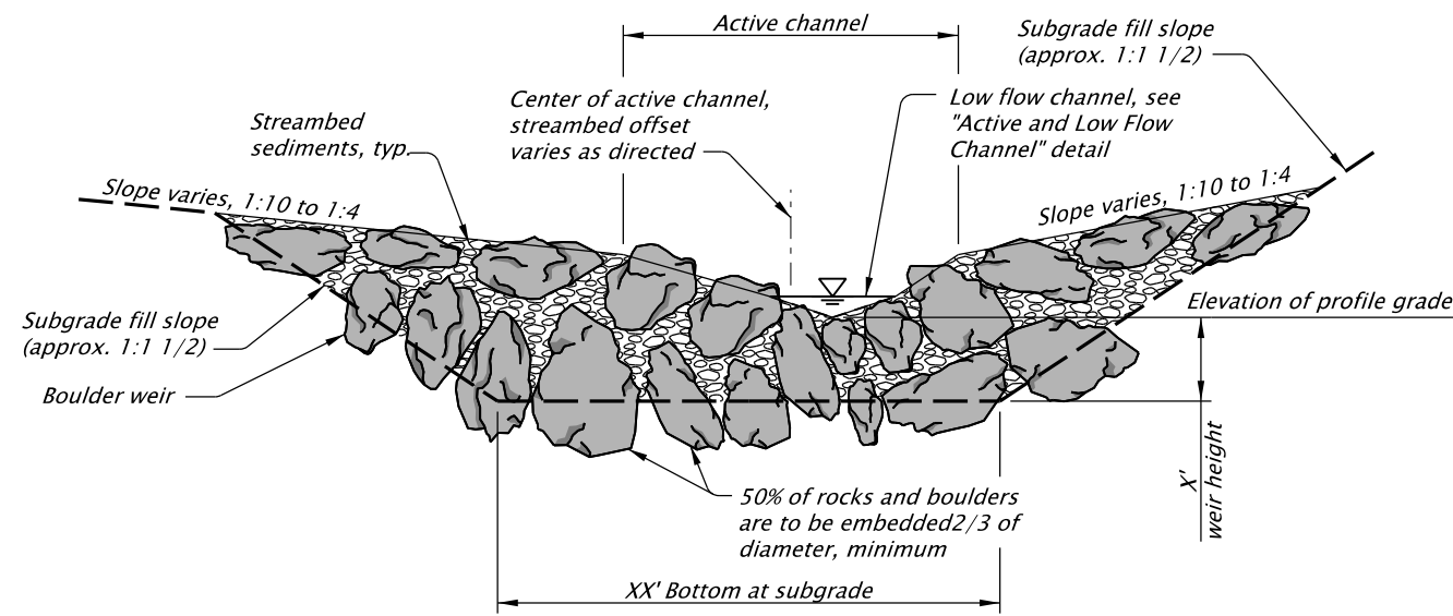
SECTION AT WEIRS
