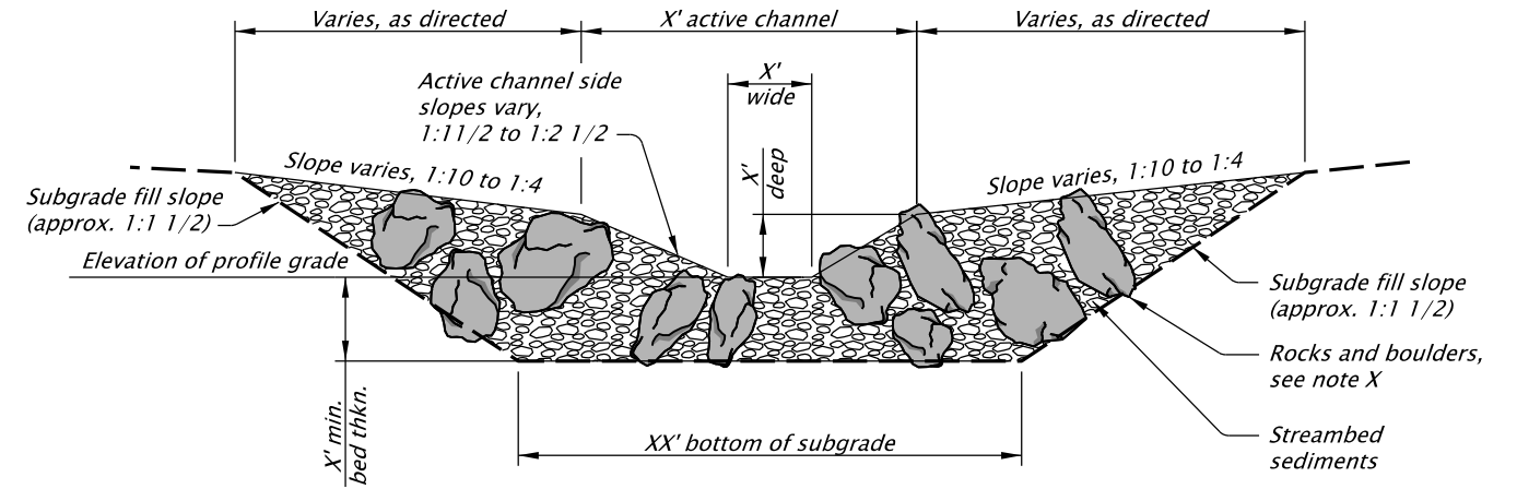
SECTION AT TANGENTS
