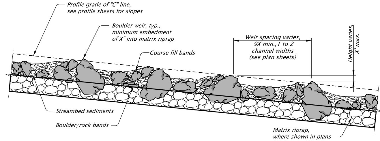
CASCAD / STEP POOL PROFILE AT CENTERLINE 3% TO 5% NOT TO SCALE
