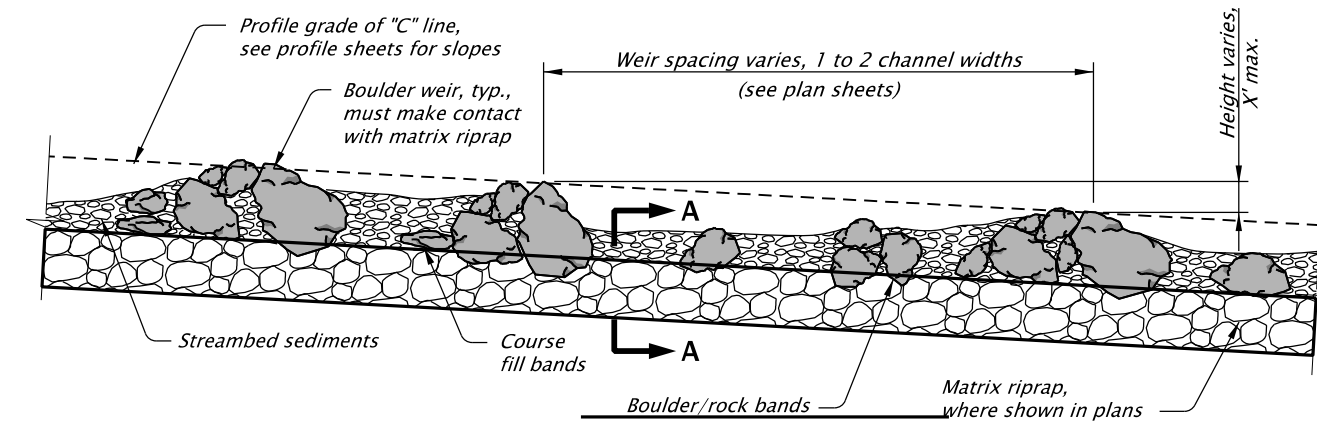
CASCAD / STEP POOL PROFILE AT CENTERLINE < 3% NOT TO SCALE
