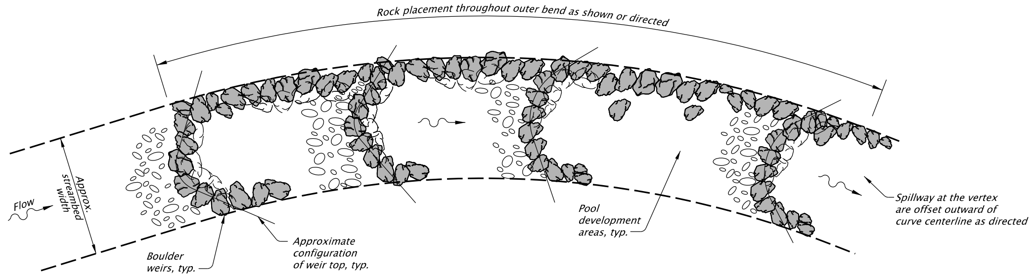
STREAM CHANNEL BOULDER AND ROCK PLACEMENT THROUGH BENDS NOT TO SCALE
