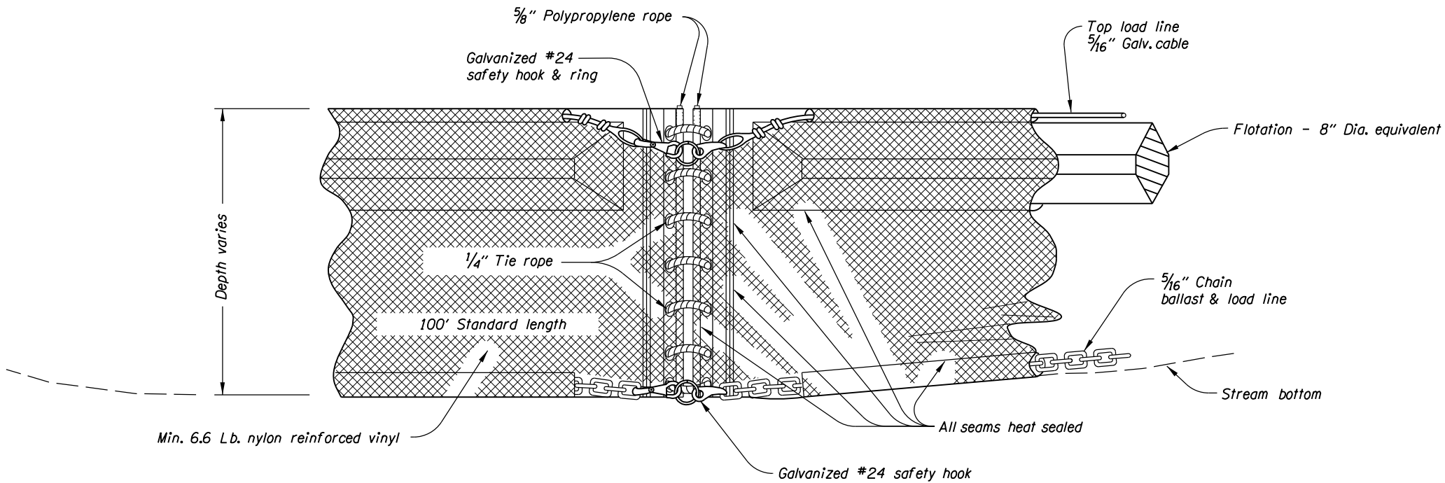
ANCHOR ASSEMBLY
