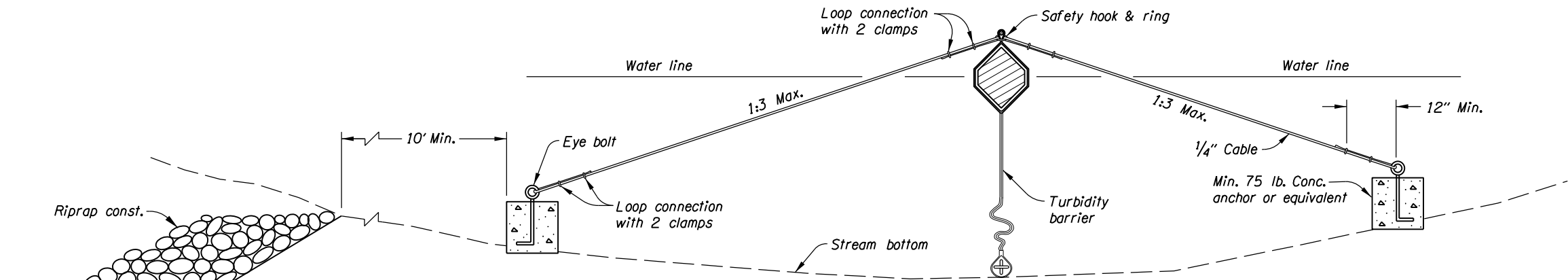
SIDE VIEW
