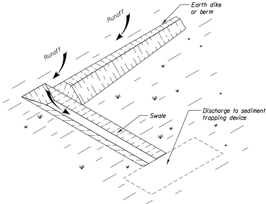
DIVERSION DIKE/SWALE
