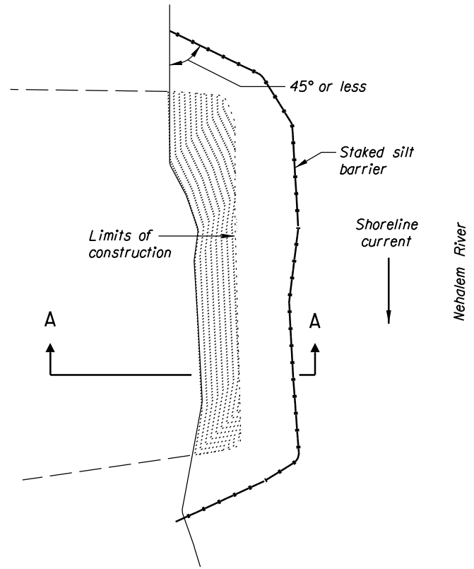
PLAN VIEW EFFECTIVE STAKED SILT BARRIER DEPLOYMENT CONFIGURATION
