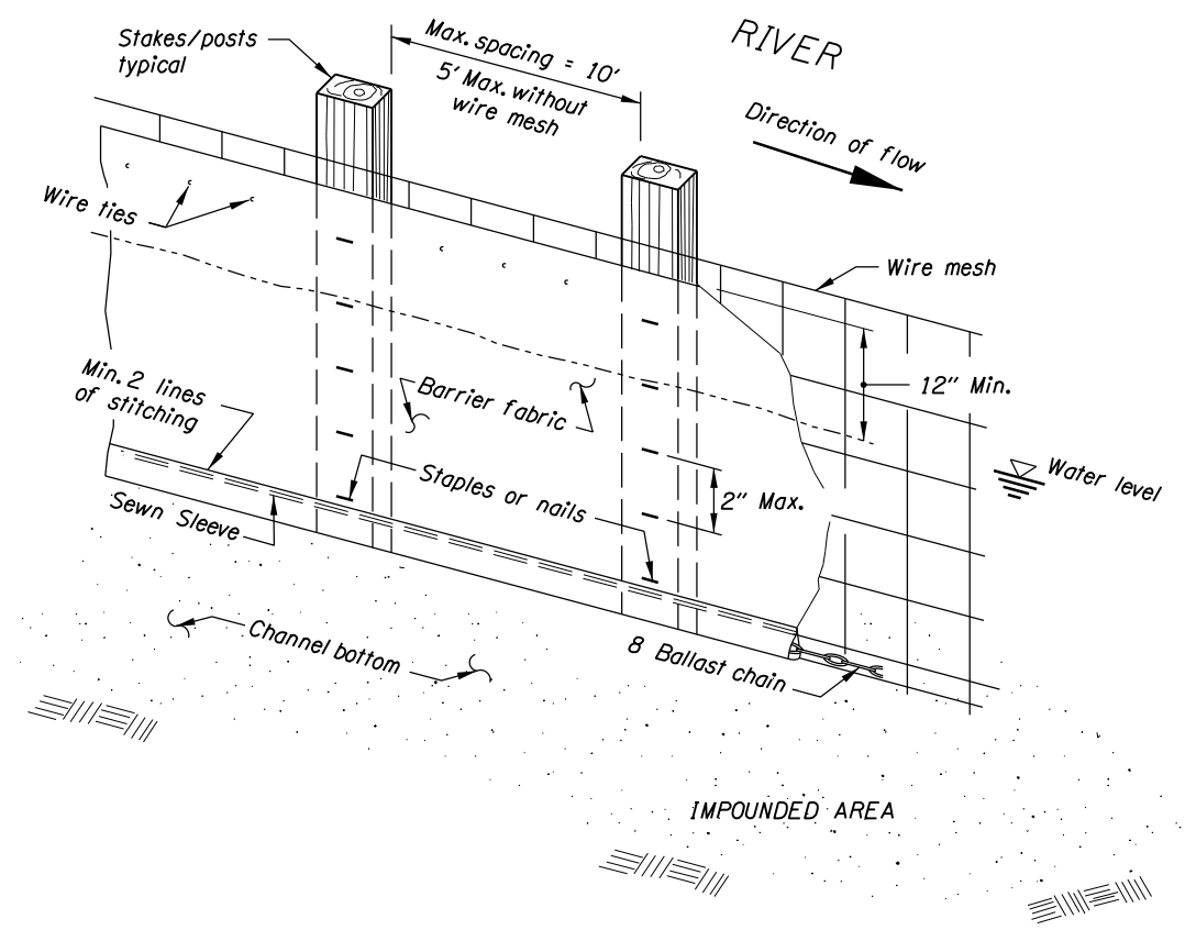
TYPICAL CONSTRUCTION OF A STAKED SILT BARRIER Not to scale
