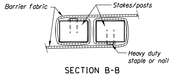
RECOMMENDED METHOD OF JOINING SECTIONS OF THE STAKED BARRIER Not to scale
