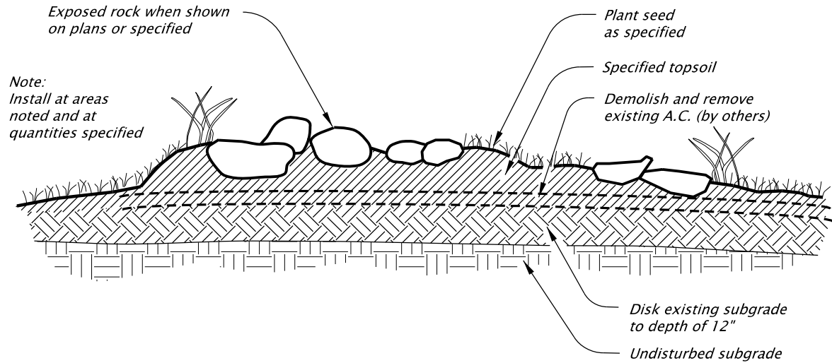
TYPICAL ROADBED REVEGETATION
