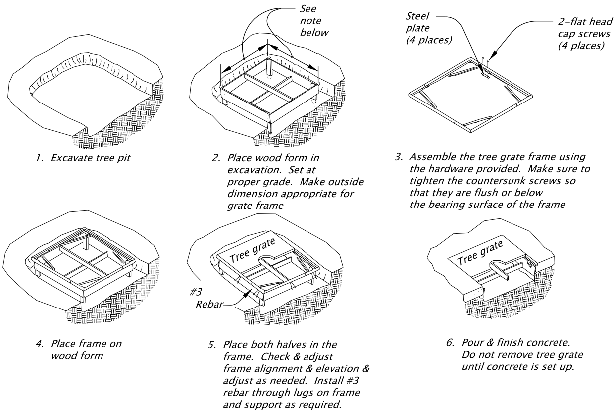
TREE GRATE INSTALLATION Refer to manufacturers recommendation for additional installation details.
