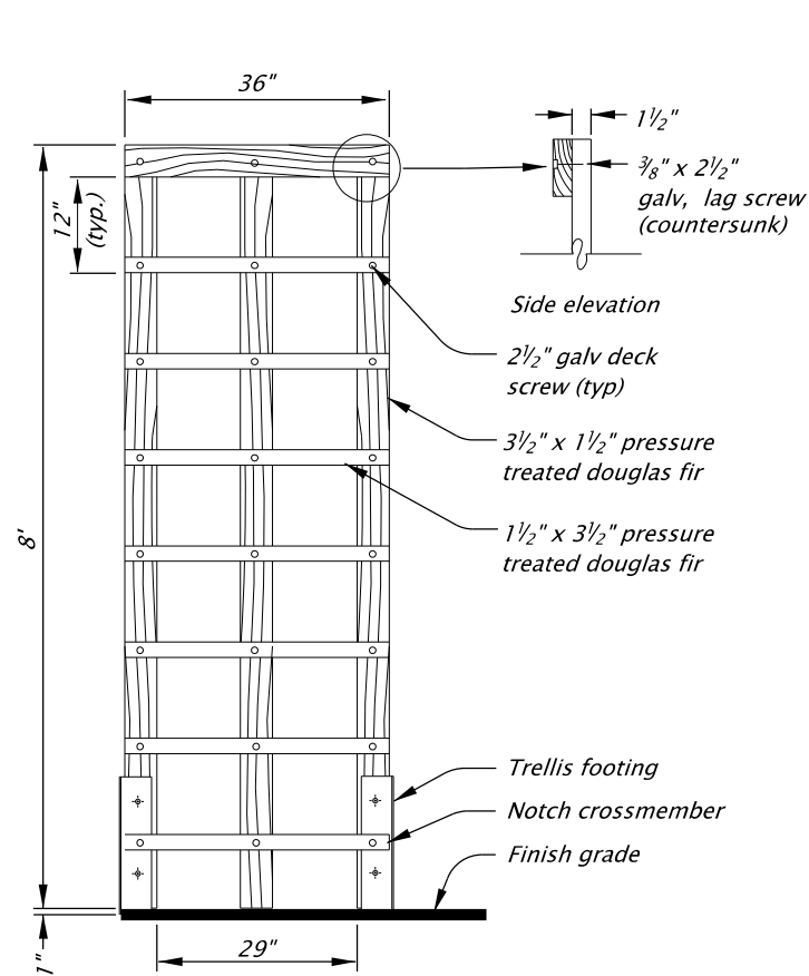
TRELLIS ELEVATION
