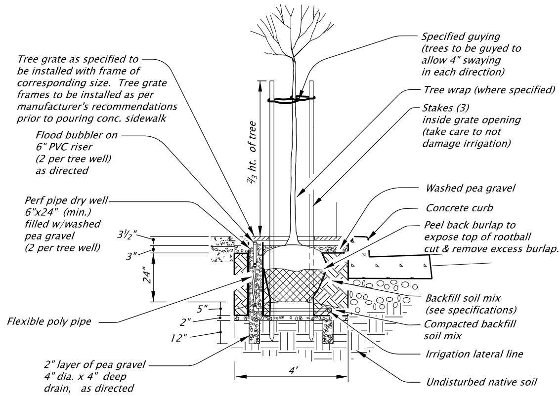
TREE GRATE & IRRIGATION AT TREE WELL
