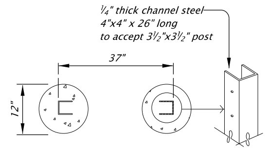
TRELLIS FOOTING PLAN
