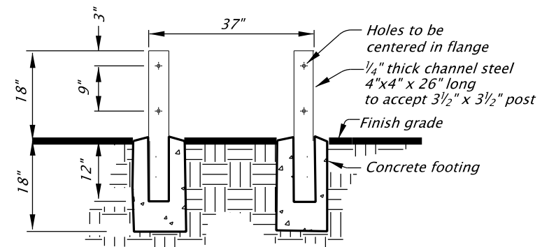
TRELLIS FOOTING SECTION
