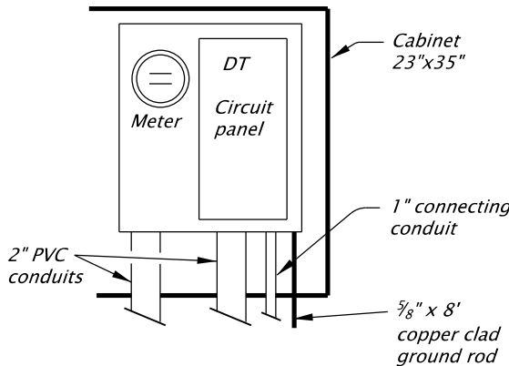
ELECTRICAL SERVICE
