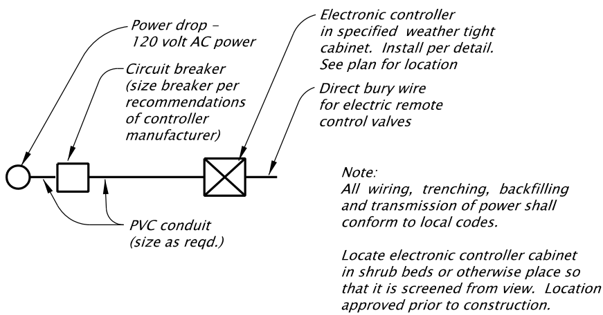
ELECTRICAL CONNECTION SCHEMATIC
