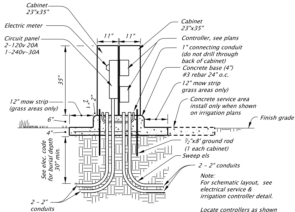
CONTROLLER SECTION
