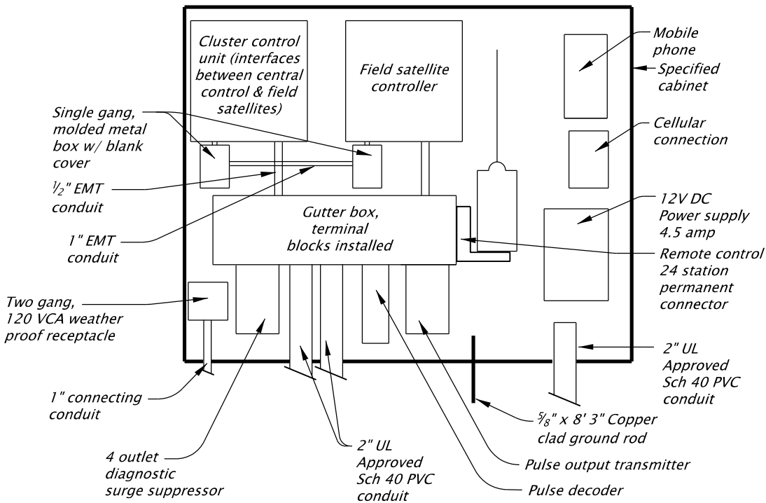
CONTROLLER LAYOUT FOR WEATHERSTATIONS
