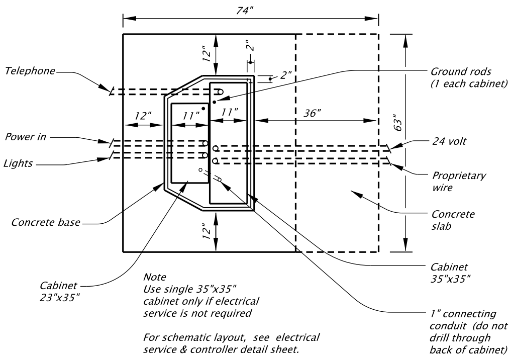
CONTROLLER PLAN
