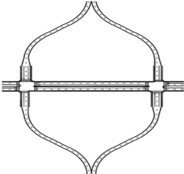
Quadrant roadway
