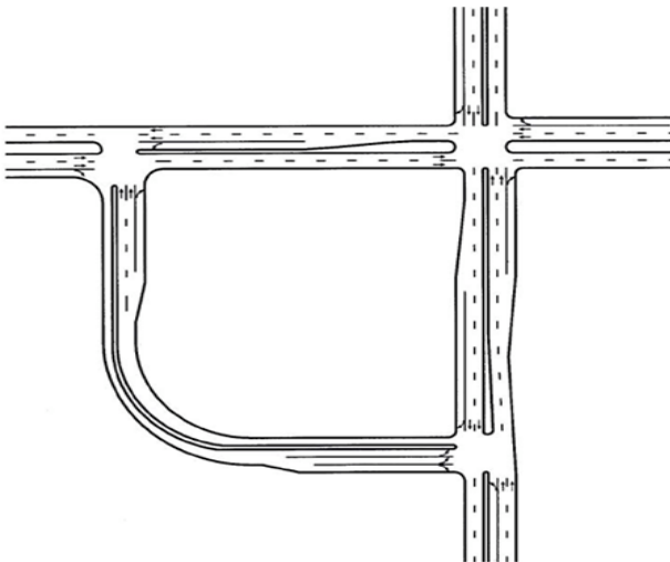
Quadrant roadway
