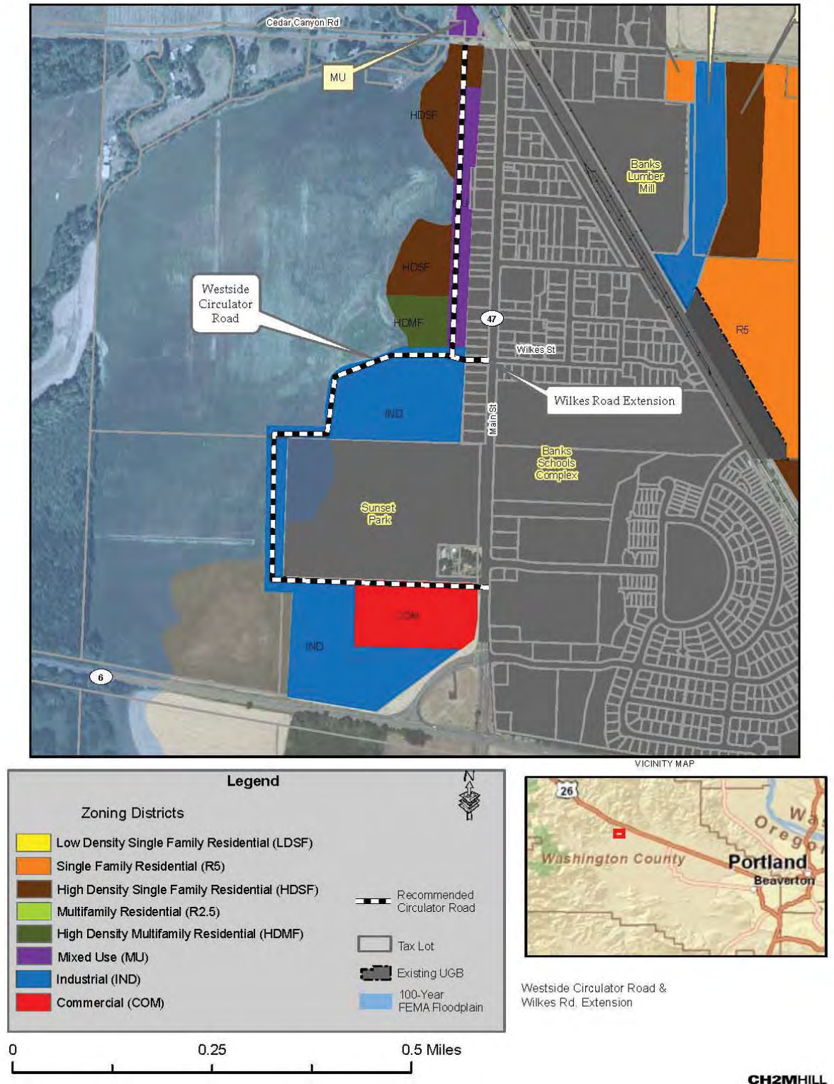
FIGURE 13: CONCEPT #8 – WESTSIDE CIRCULATOR ROAD
