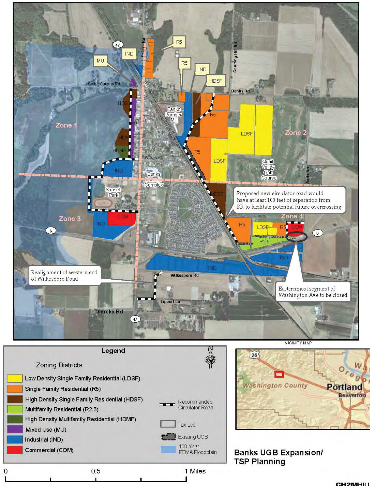
FIGURE 5: CONCEPTUAL UGB EXPANSION AREA ROADWAY CIRCULATION USED FOR TRIP GENERATION ESTIMATION
